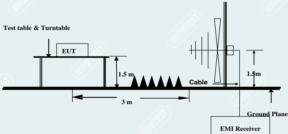
Figure 6.8-1: 30MHz-1000MHz measurement arrangement
