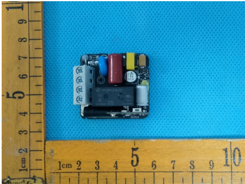
Front view of power PCB
