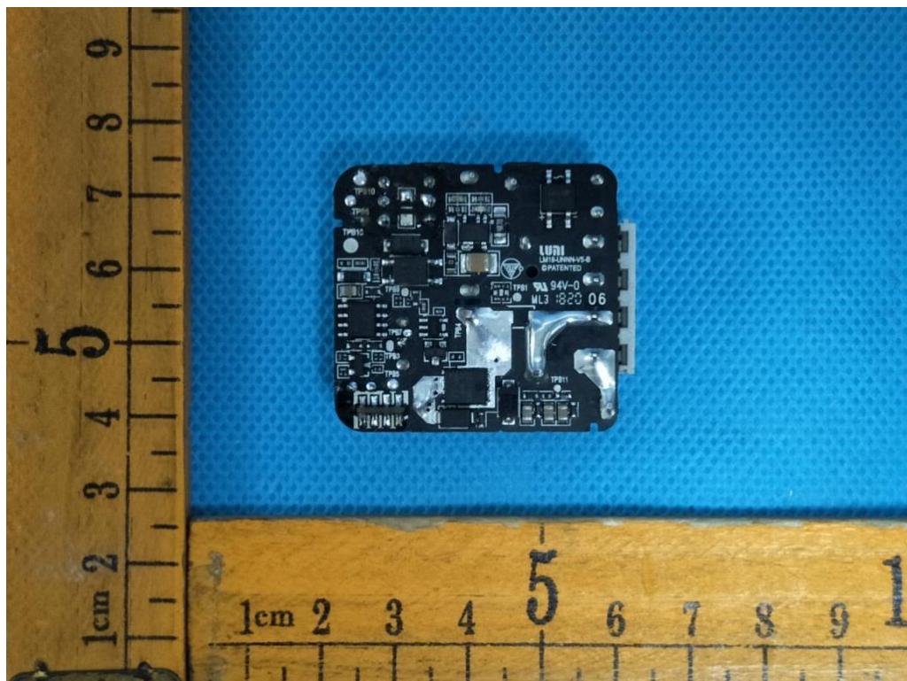
Back view of power PCB
