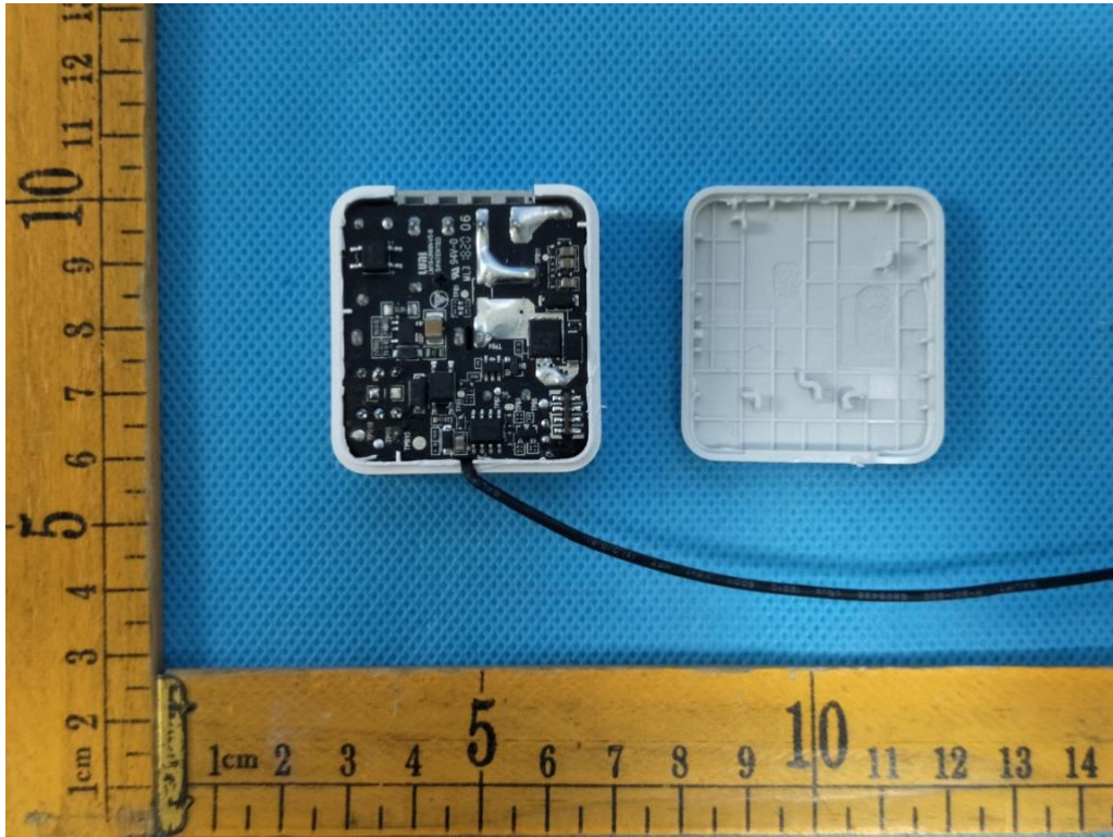
Internal view of switch
