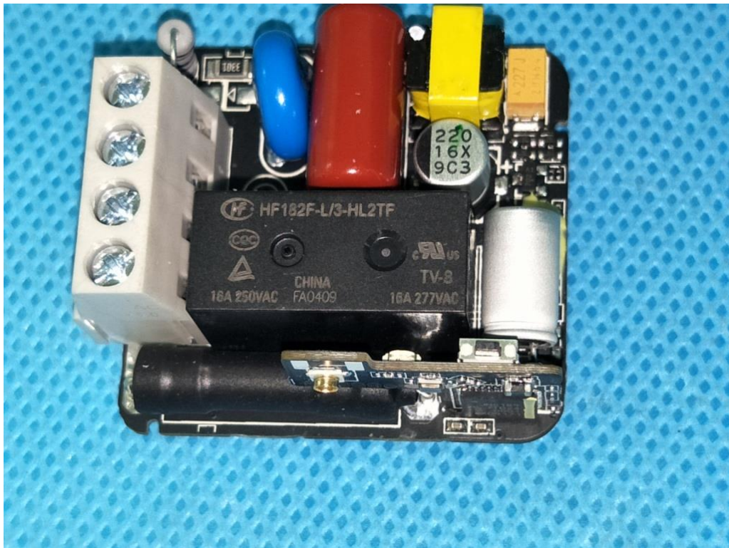
Close-up view of relay
