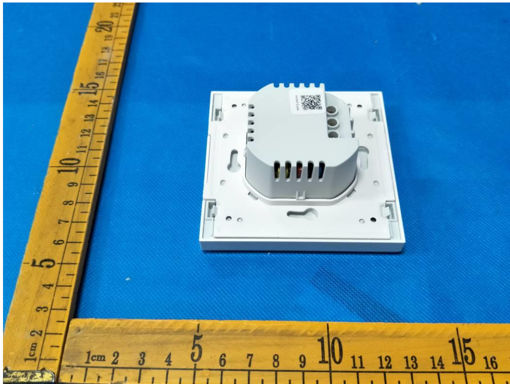
Photo 5. External view of the specimen
