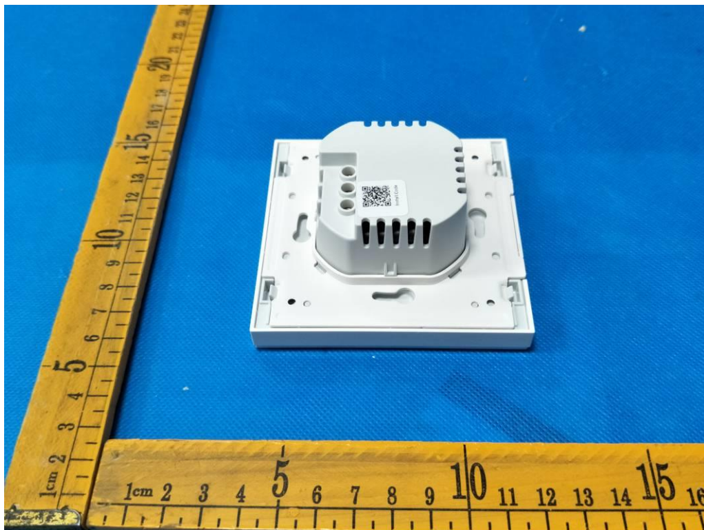
Photo 6. External view of the specimen
