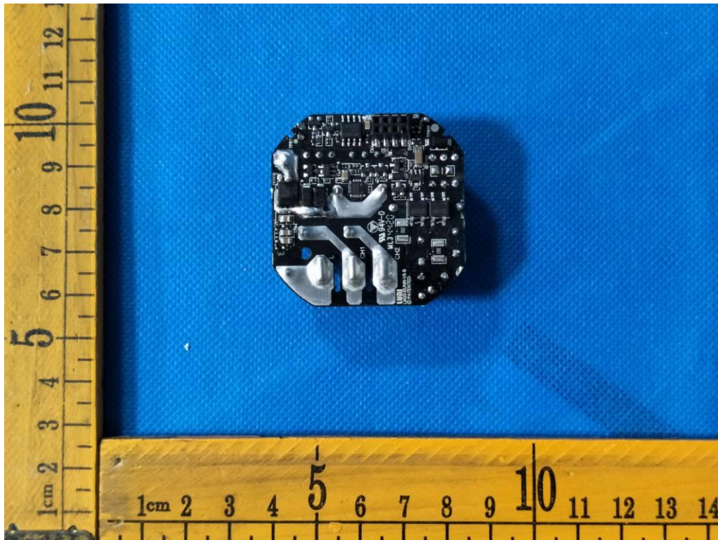
Photo 13. Internal view of the specimen
