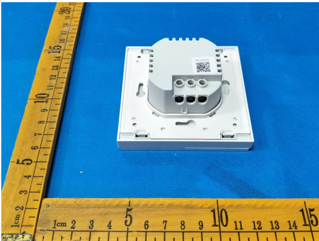
Photo 4. External view of the specimen
