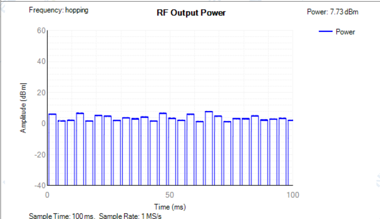
Power NVNT 1-DH5 2402MHz Ant1
