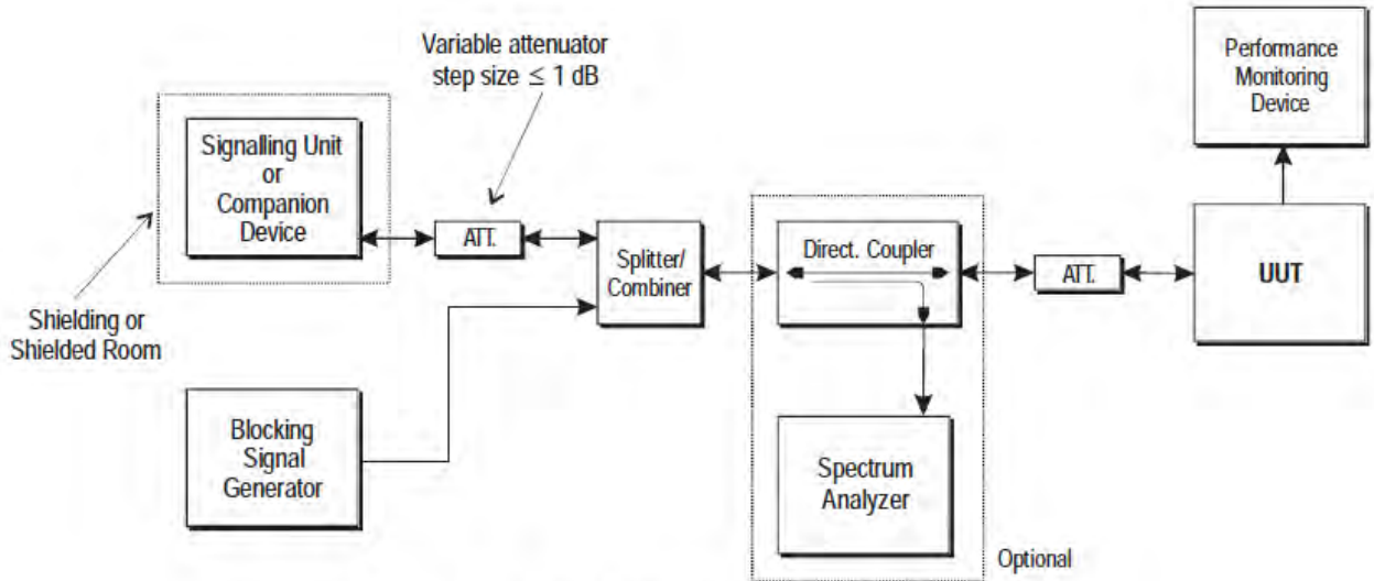
Figure 14: Test Set-up for receiver blocking
