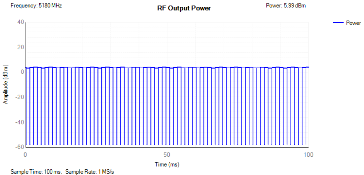
Power NVNT 802.11n(HT20) 5180MHz
