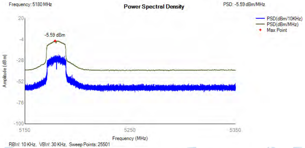
PSD NVNT 802.11n(HT20) 5180MHz
