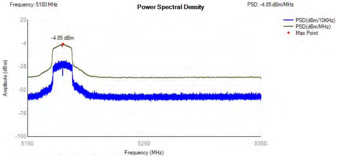
PSD NVNT 802.11n(HT20) 5180MHz
