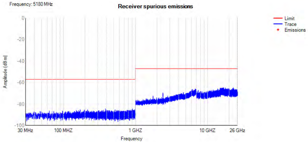
Rx. Spurious NVNT 802.11n(HT20) 5180MHz
