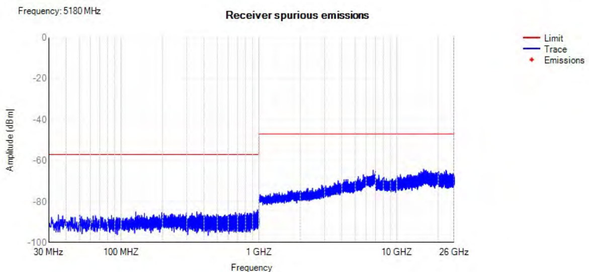
Rx. Spurious NVNT 802.11a 5180MHz
