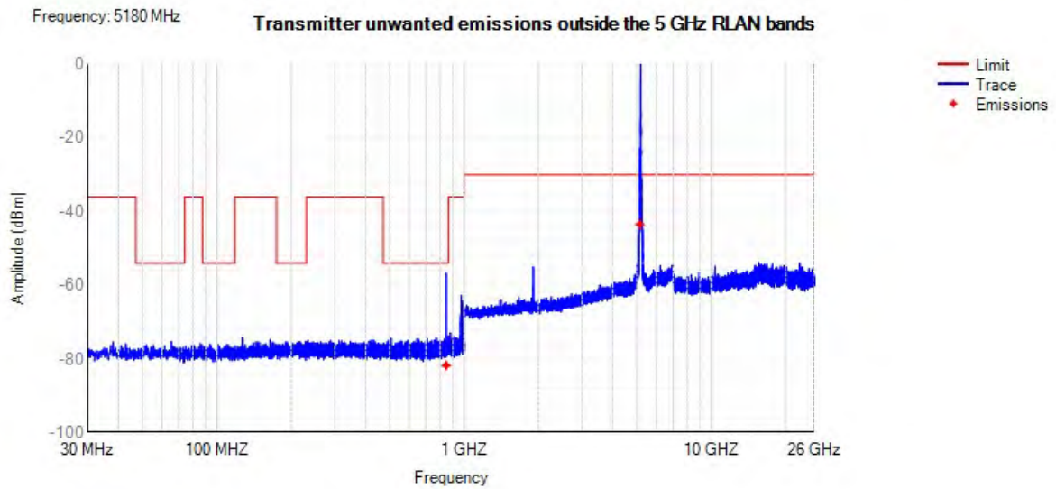
Tx. Spurious NVNT 802.11ac20 5180MHz
