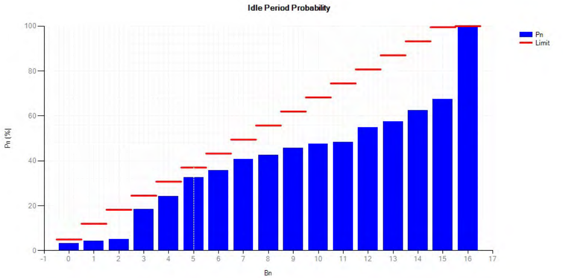
Idle Period Probability NVNT 802.11n(HT40) 5190MHz
