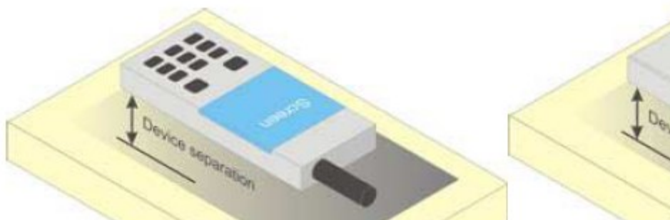
Figure 6.1 – Test positions for Body-worn device
