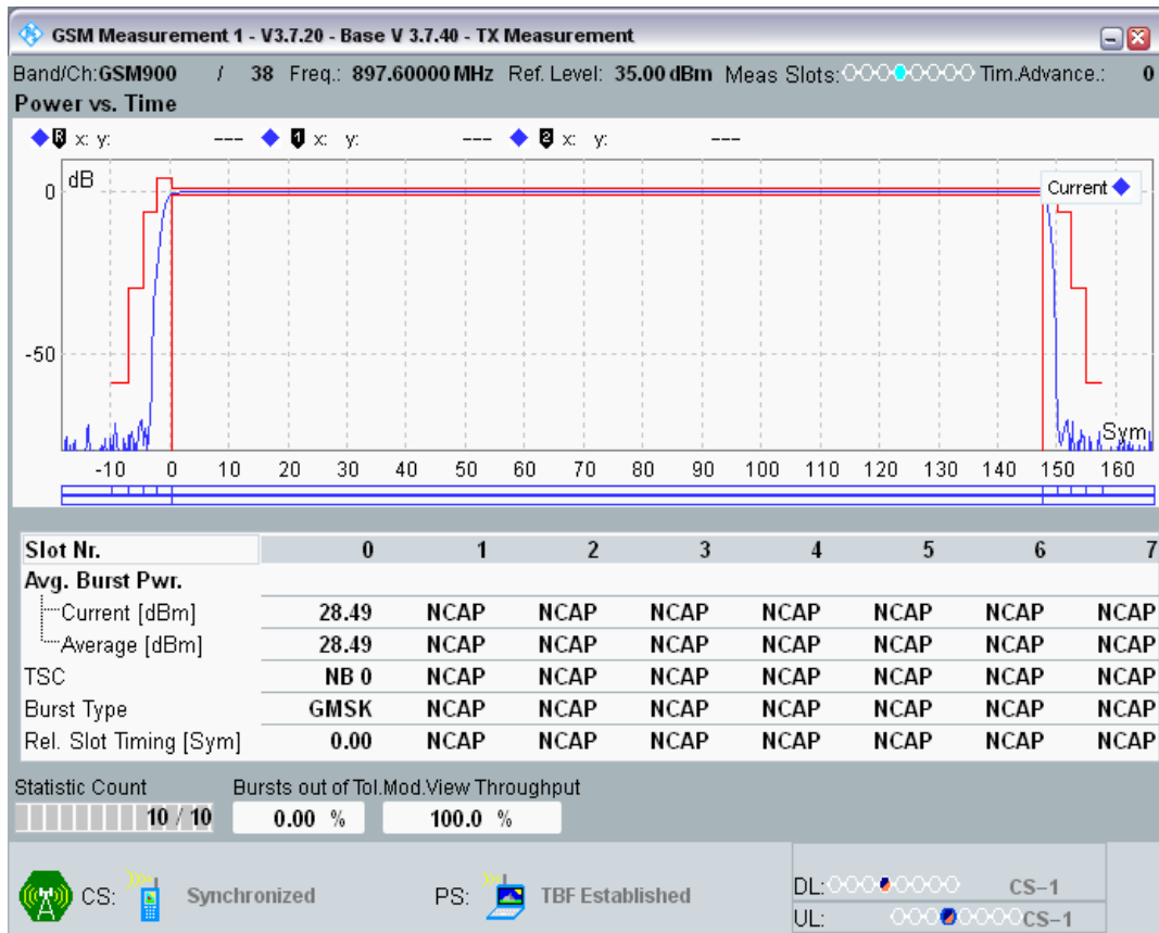
GPRS900 Channel=38 Gamma=7;7;7
