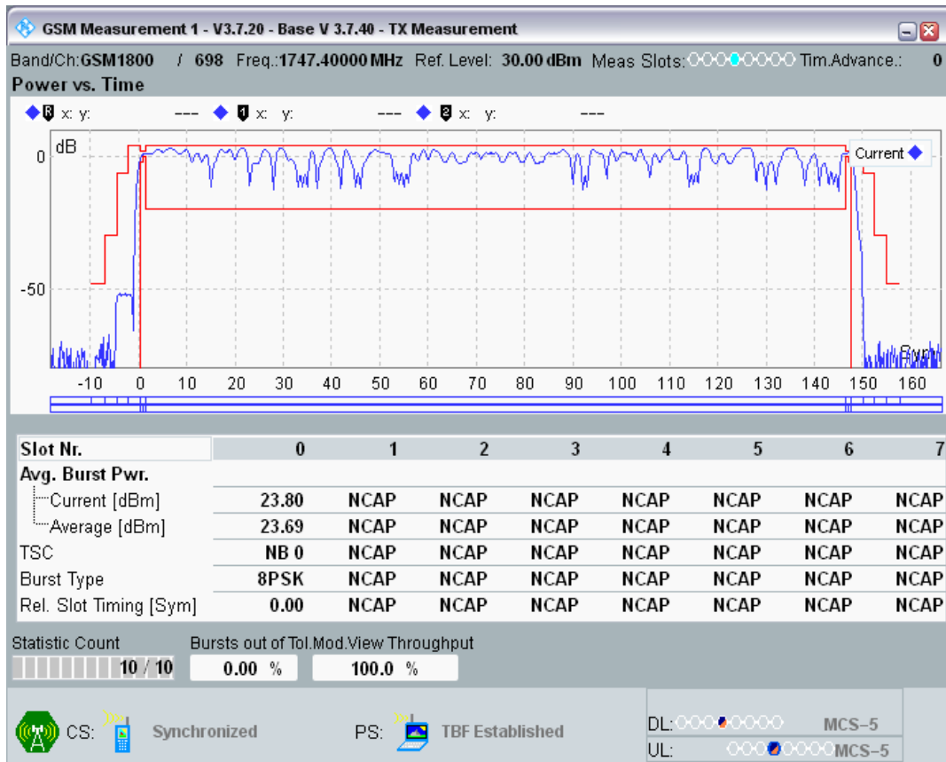
EGPRS1800 Channel=698 Gamma=7;7;7;7
