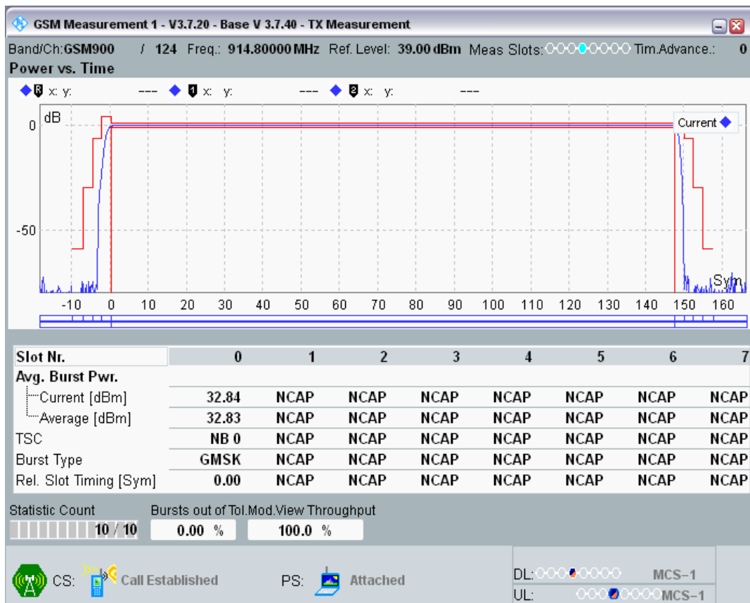
GSM900 Channel=124 PCL=7
