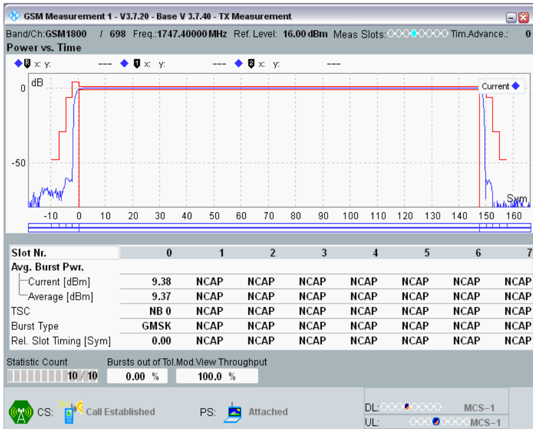
GSM1800 Channel=698 PCL=11
