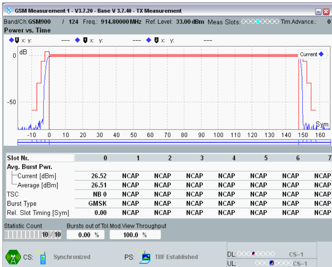
GPRS900 Channel=124 Gamma=7;7;7;7
