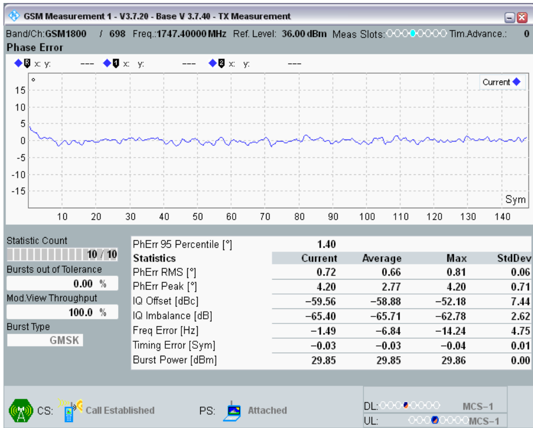
GSM1800 Channel=698 PCL=0 RA130 @RACH
