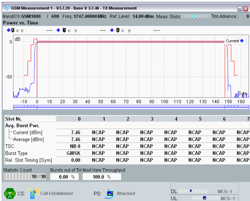
GSM1800 Channel=698 PCL=12
