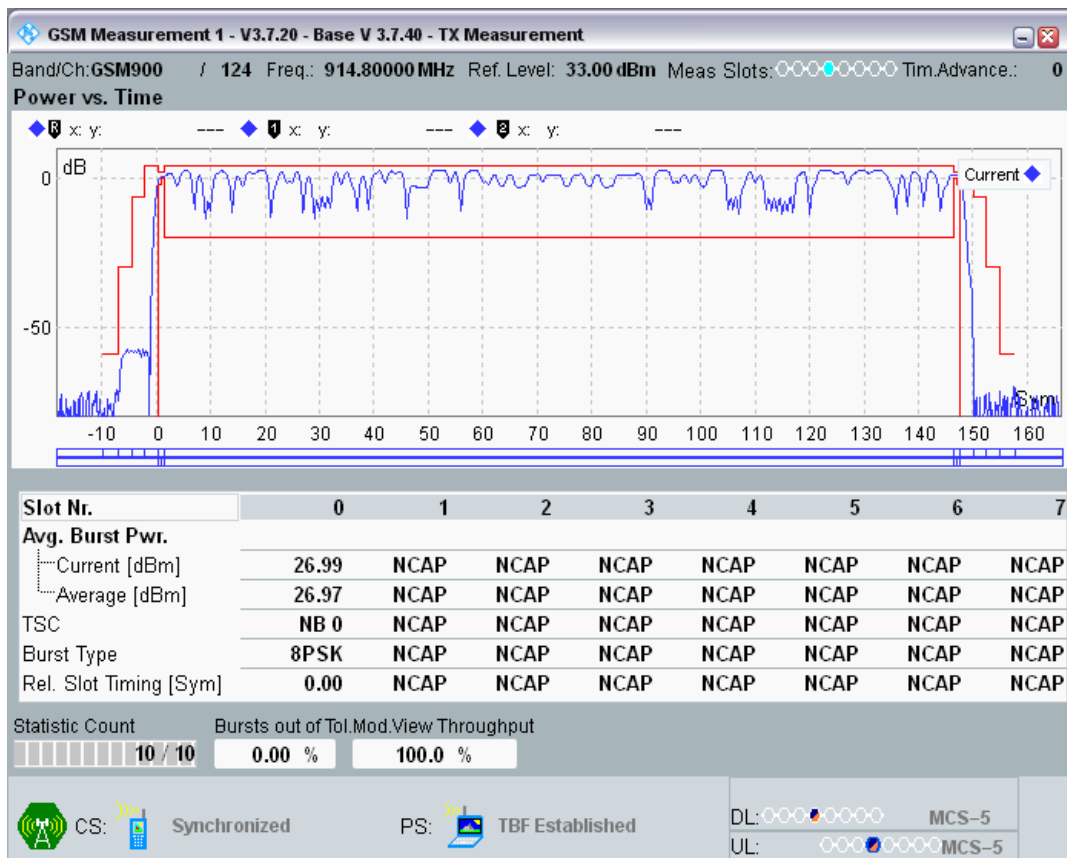
EGPRS900 Channel=124 Gamma=7;7;7;7
