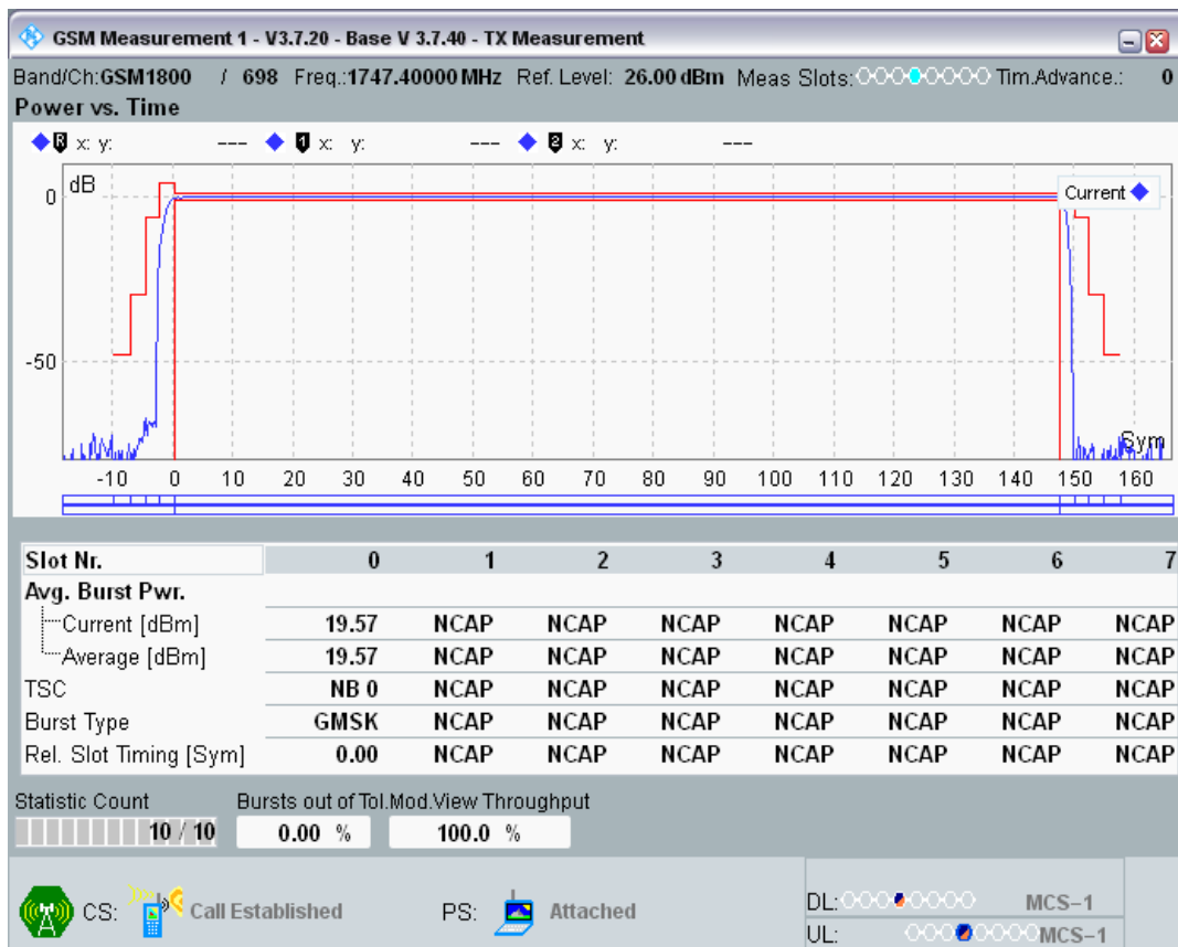
GSM1800 Channel=698 PCL=6
