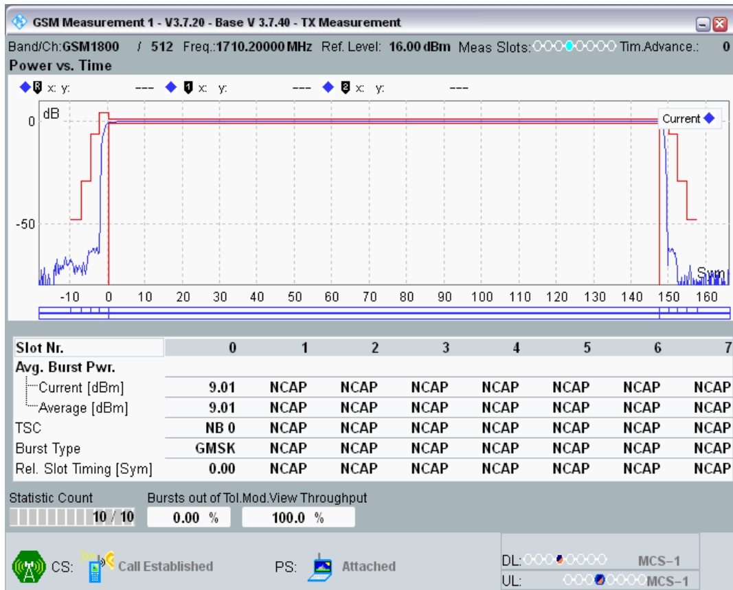
GSM1800 Channel=512 PCL=12
