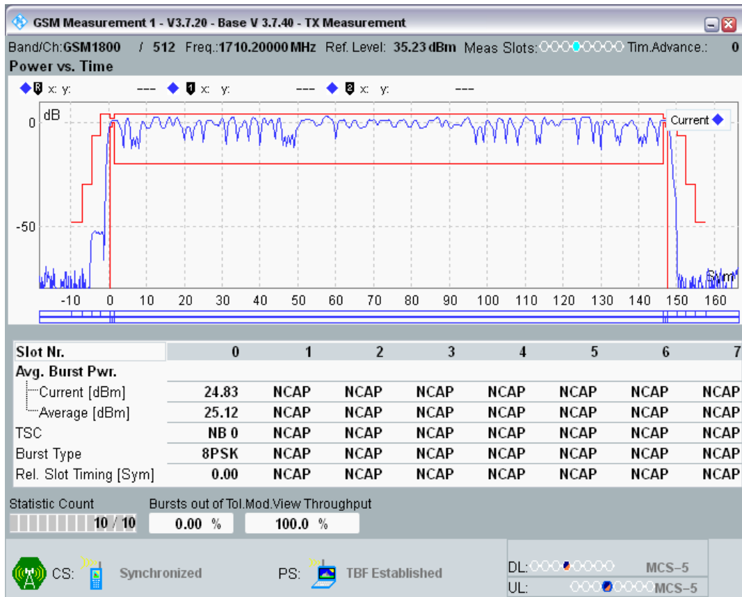
EGPRS1800 Channel=512 Gamma=7;7;7;7
