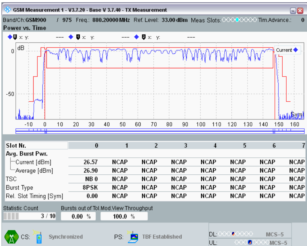
EGPRS900 Channel=975 Gamma=7;7;7
