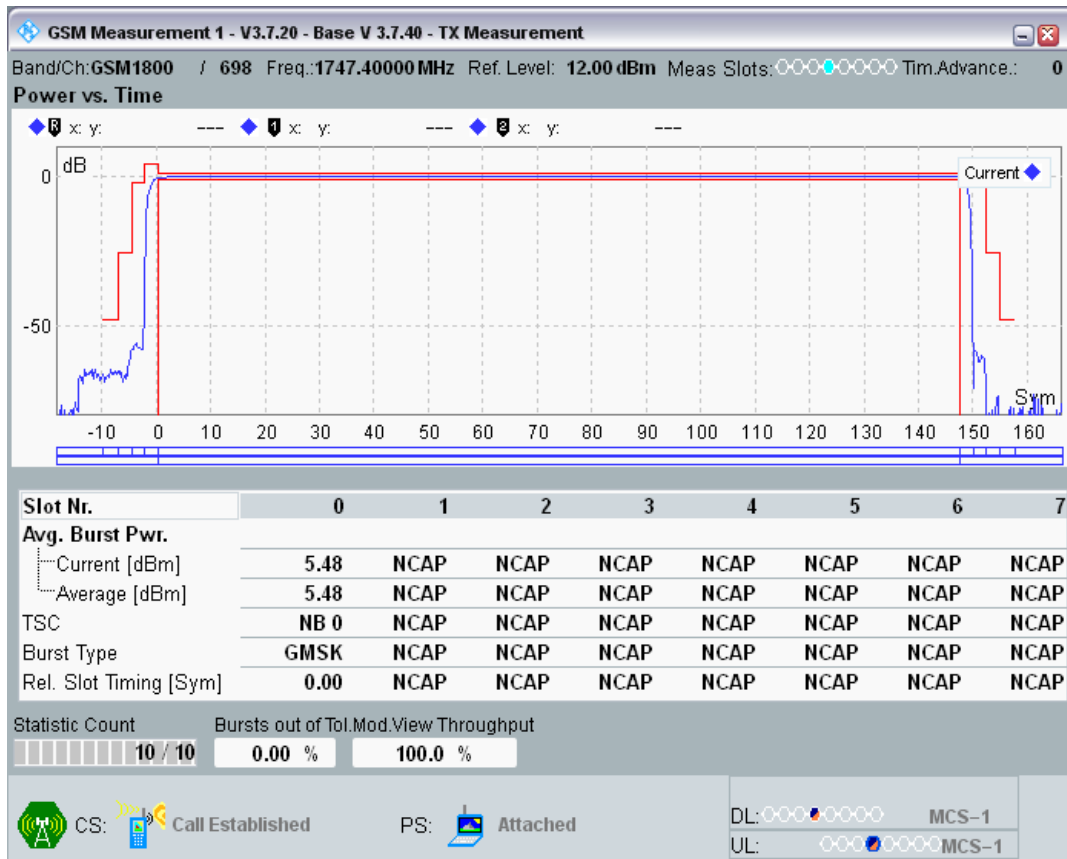
GSM1800 Channel=698 PCL=13
