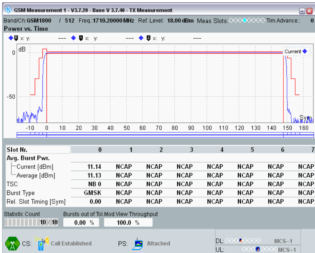
GSM1800 Channel=512 PCL=10
