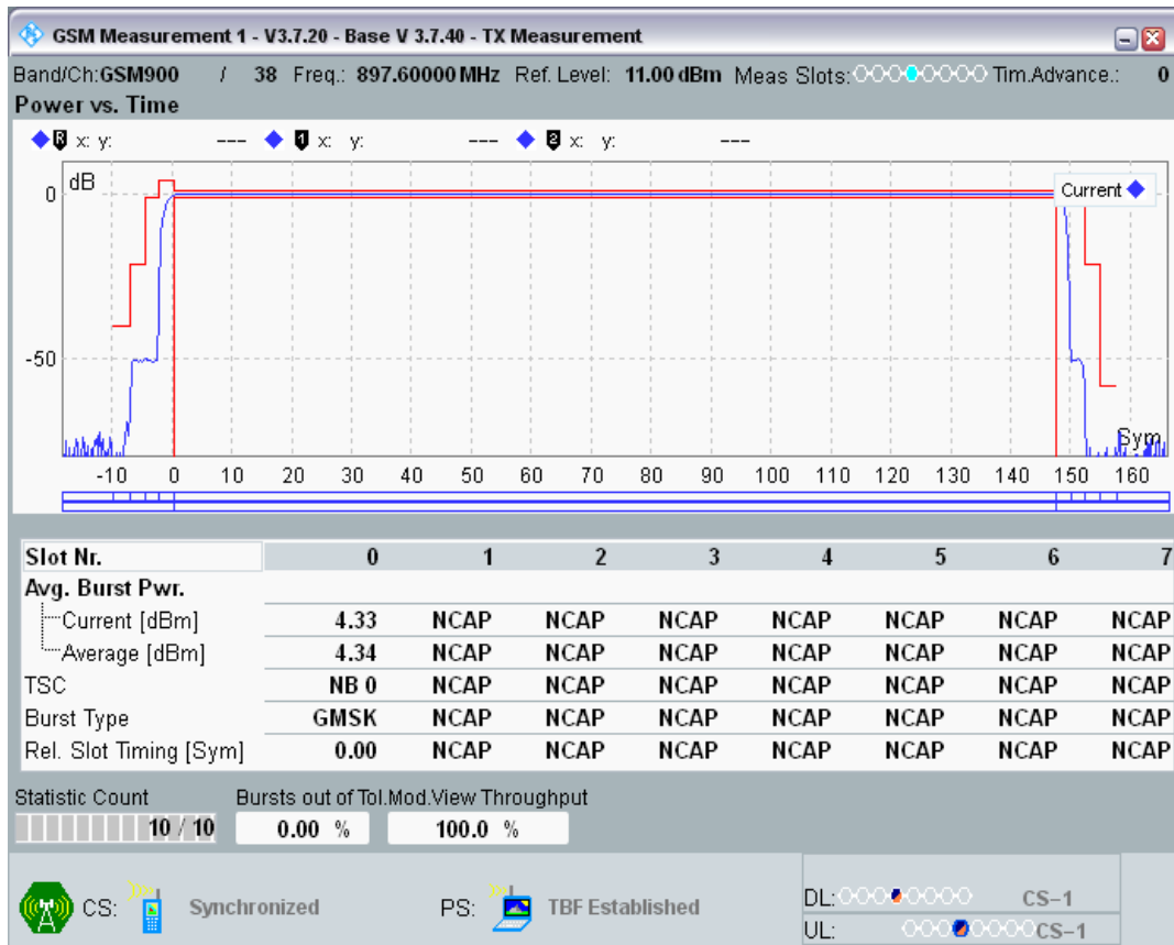
GPRS900 Channel=124 Gamma=4;4;4;4
