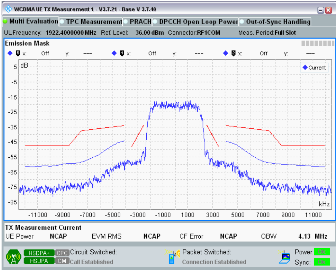
HSUPA Band1 Channel=9612 Subtest2
