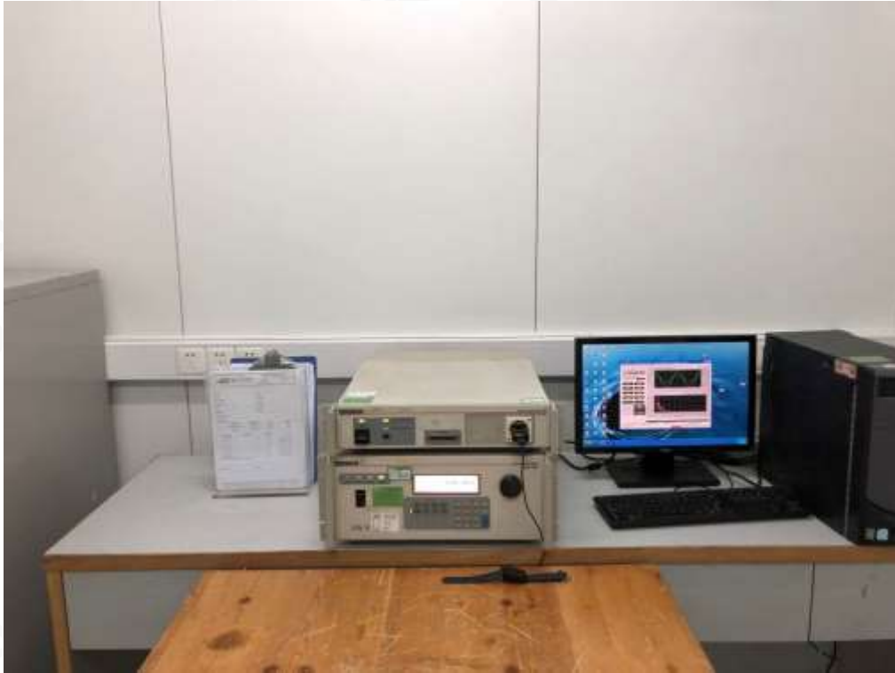
EFT / SURGE / DIPS IMMUNITY TEST
