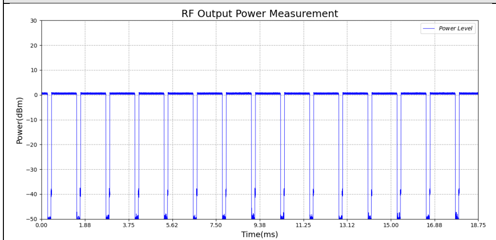
Test_Graph_LE2M_TX_2440_2Mbps_Power_NT
