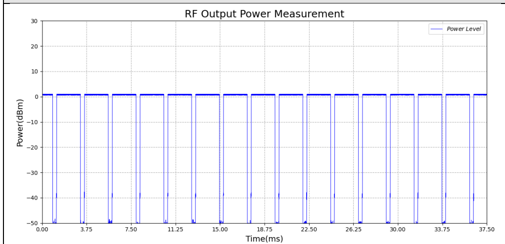
Test_Graph_LE1M_TX_2440_1Mbps_Power_NT
