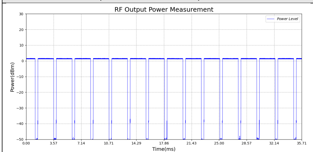
Test_Graph_LE1M_TX_2480_1Mbps_Power_NT
