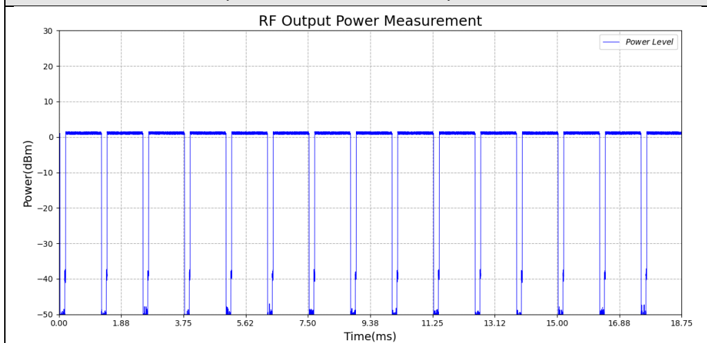
Test_Graph_LE2M_TX_2480_2Mbps_Power_NT
