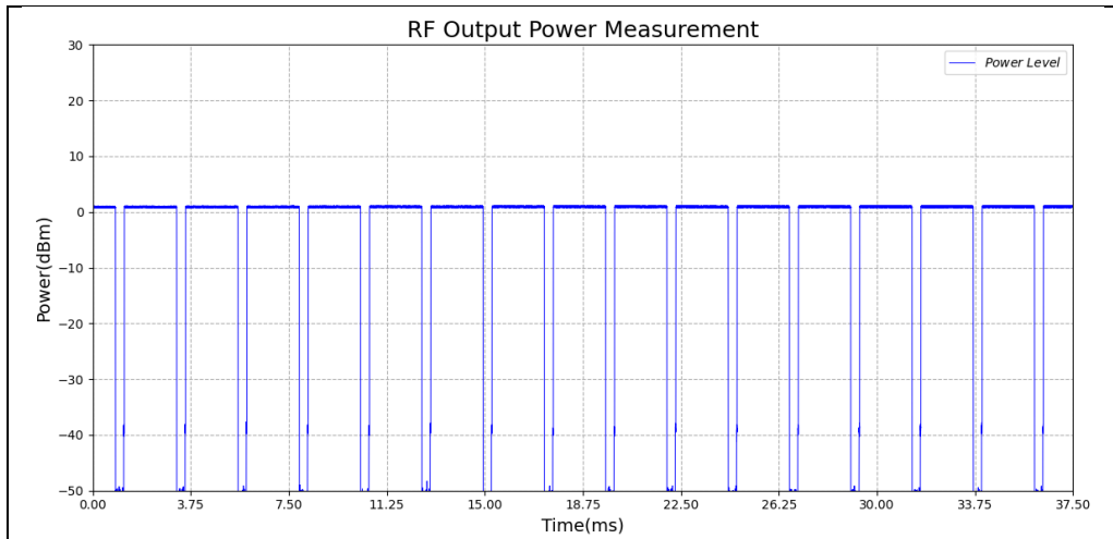
Test_Graph_LE1M_TX_2402_1Mbps_Power_NT
