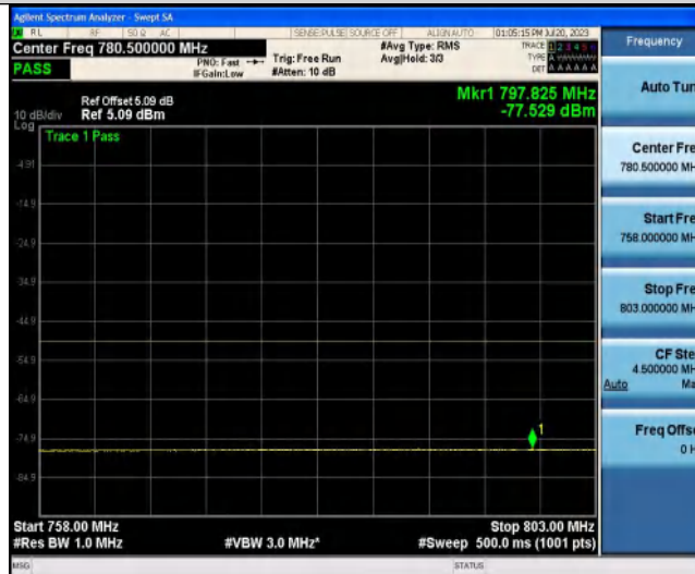
NTNV-Band3-1.4MHz-QPSK-19207-6RB#0-791~821-1000-3000
