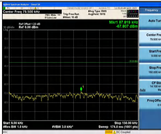
NTNV-Band3-20MHz-QPSK-19575-1RB#99-0.15~30-10-30
