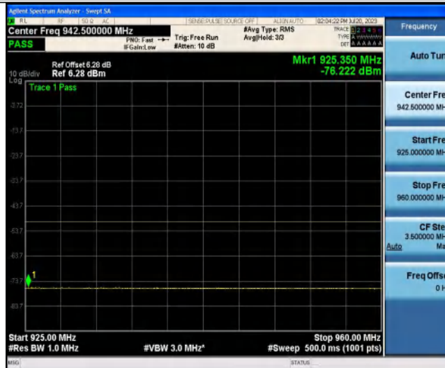
NTNV-Band3-5MHz-QPSK-19925-1RB#24-1452~1496-1000-3000
