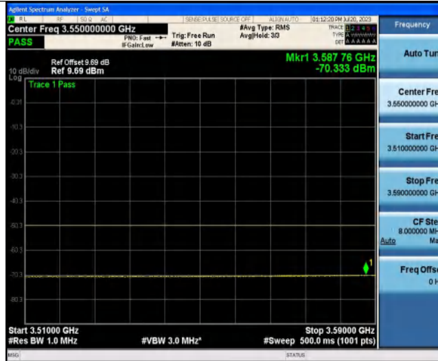
NTNV-Band3-1.4MHz-QPSK-19575-1RB#0-3600~3800-1000-3000
