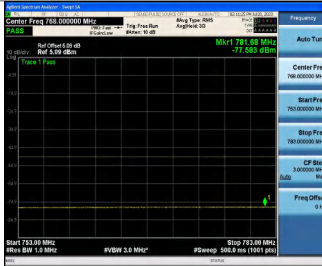
NTNV-Band3-5MHz-QPSK-19925-25RB#0-758~803-1000-3000
