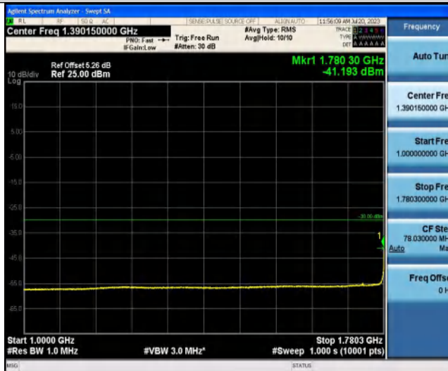
NTNV-Band3-1.4MHz-QPSK-19943-1RB#0-1788.3~3000-1000-3000
