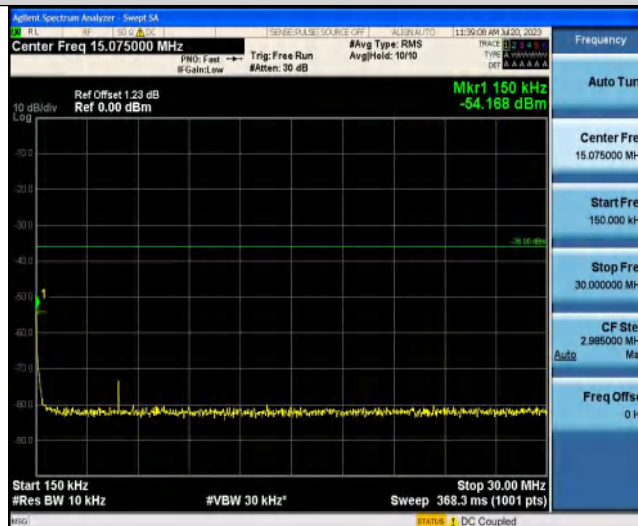
NTNV-Band3-20MHz-QPSK-19850-1RB#0-30~1000-100-300
