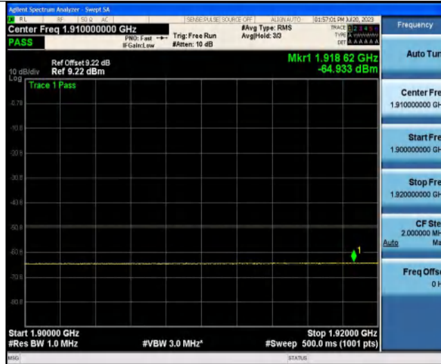
NTNV-Band3-5MHz-QPSK-19575-25RB#0-2110~2170-1000-3000
