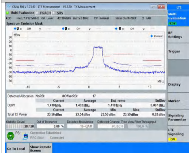
NTNV-Band3-5MHz-16QAM-19575-8RB#0
