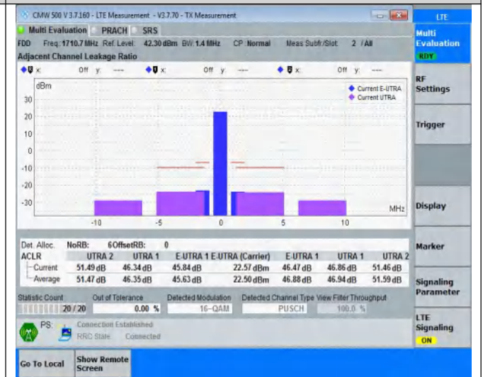
NTNV-Band3-1.4MHz-16QAM-19575-5RB#1
