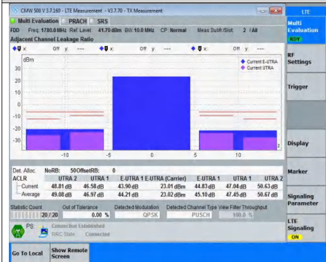
NTNV-Band3-10MHz-16QAM-19250-12RB#38
