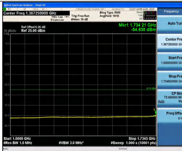
NTNV-Band3-5MHz-QPSK-19575-1RB#0-1760.5~3000-1000-3000
