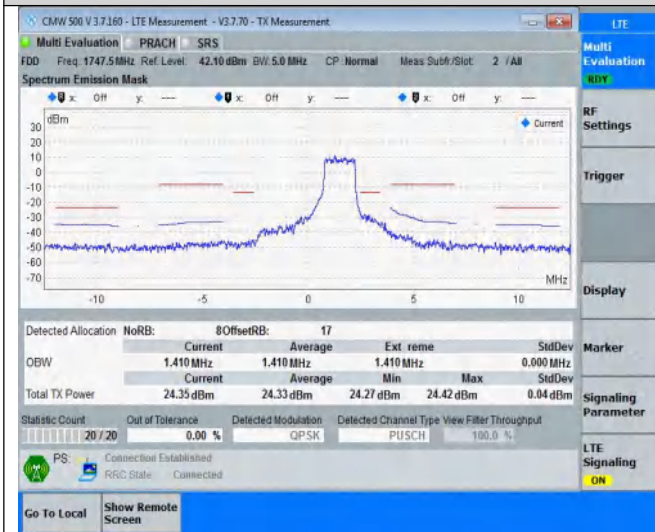
NTNV-Band3-5MHz-QPSK-19925-8RB#0
