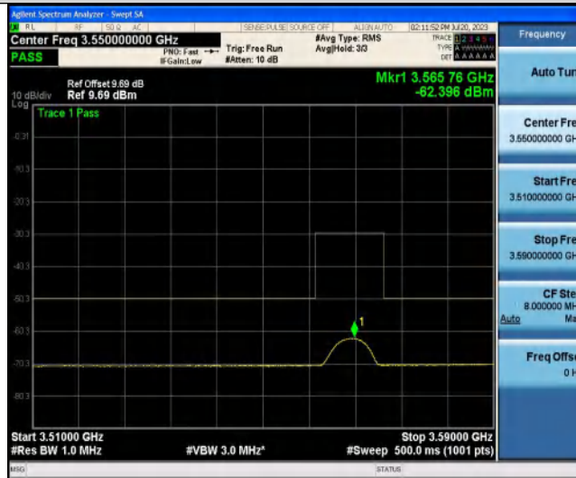
NTNV-Band3-5MHz-QPSK-19925-25RB#0-3600~3800-1000-3000
