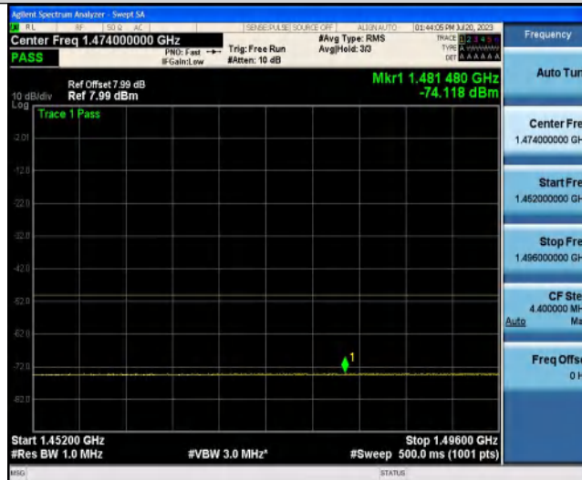
NTNV-Band3-5MHz-QPSK-19225-25RB#0-1805~1880-1000-3000
