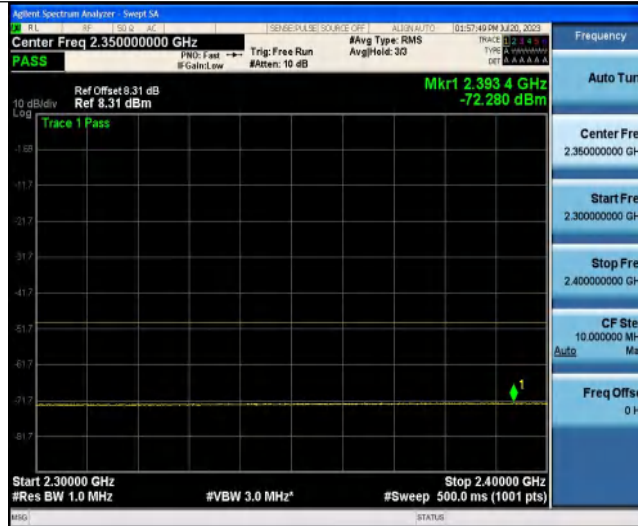
NTNV-Band3-5MHz-QPSK-19575-25RB#0-2570~2620-1000-3000
