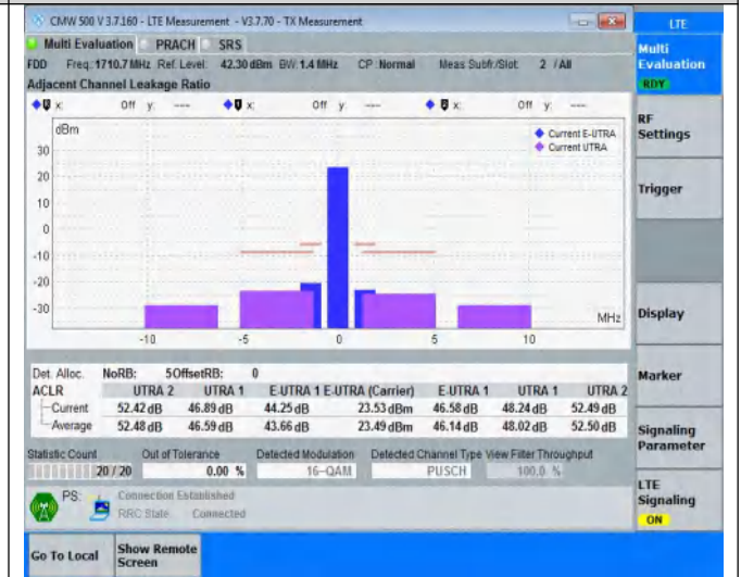
NTNV-Band3-1.4MHz-16QAM-19207-6RB#0
