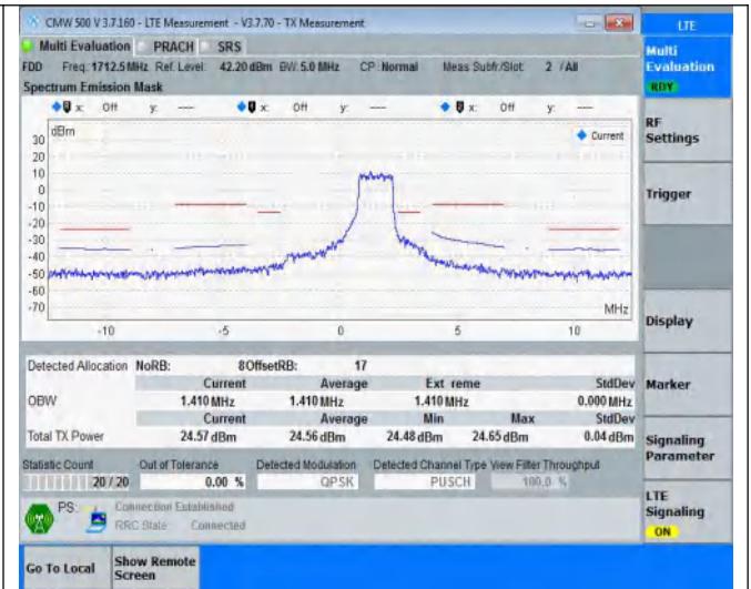
NTNV-Band3-5MHz-QPSK-19575-8RB#0
