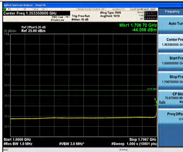
NTNV-Band3-1.4MHz-QPSK-19207-1RB#5-1714.7~3000-1000-3000
