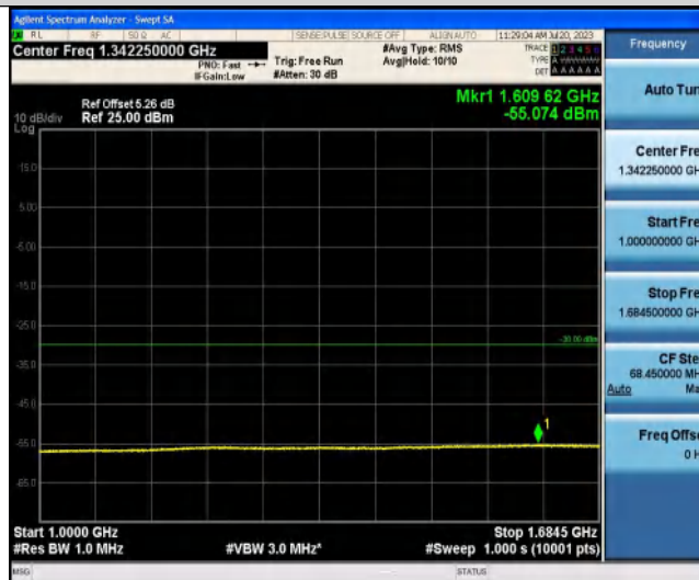
NTNV-Band3-20MHz-QPSK-19300-1RB#0-1755.5~3000-1000-3000
