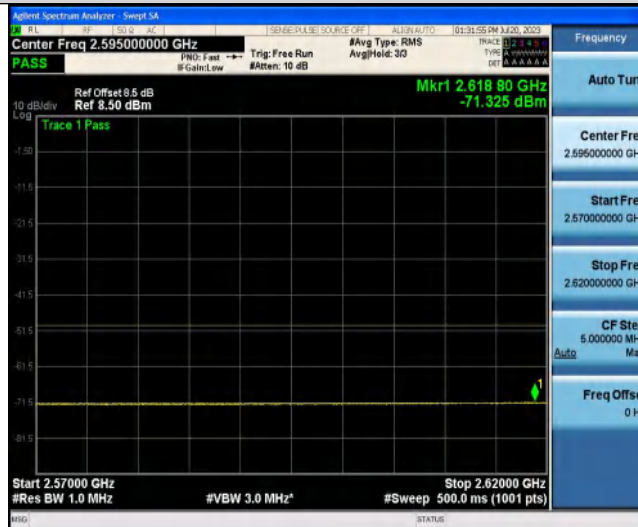
NTNV-Band3-1.4MHz-QPSK-19943-6RB#0-2620~2690-1000-3000
