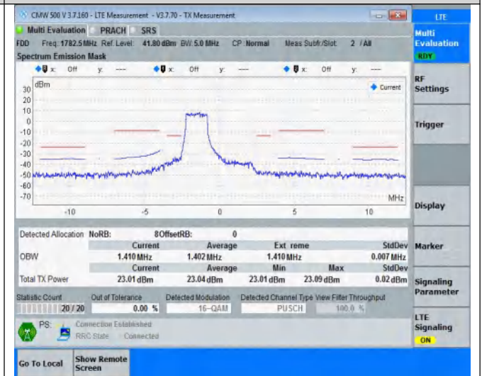
NTNV-Band3-5MHz-16QAM-19925-25RB#0
