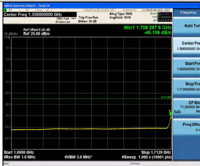
NTNV-Band3-20MHz-QPSK-19575-100RB#0-1783~3000-1000-3000
