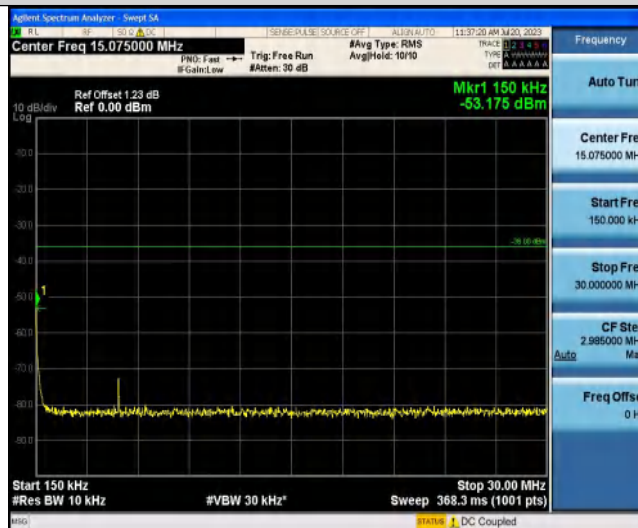
NTNV-Band3-20MHz-QPSK-19575-100RB#0-30~1000-100-300
