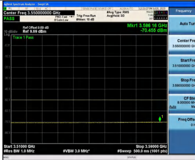
NTNV-Band3-20MHz-QPSK-19300-1RB#0-3600~3800-1000-3000
