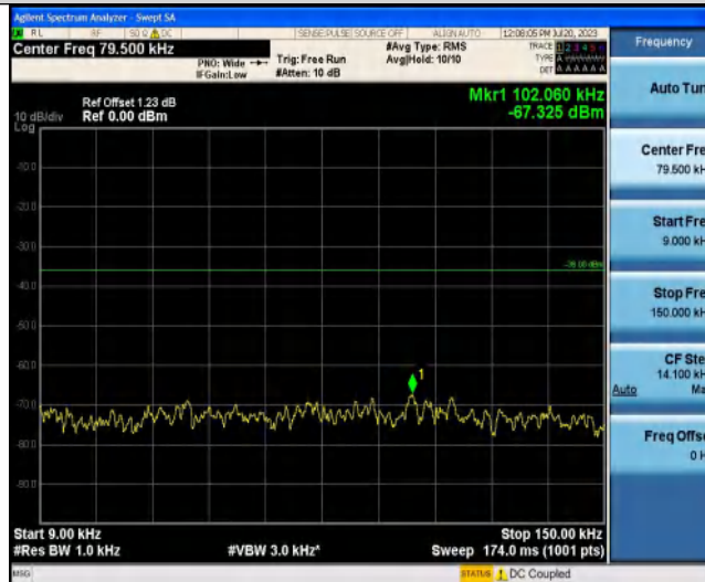
NTNV-Band3-5MHz-QPSK-19575-1RB#24-0.15~30-10-30
