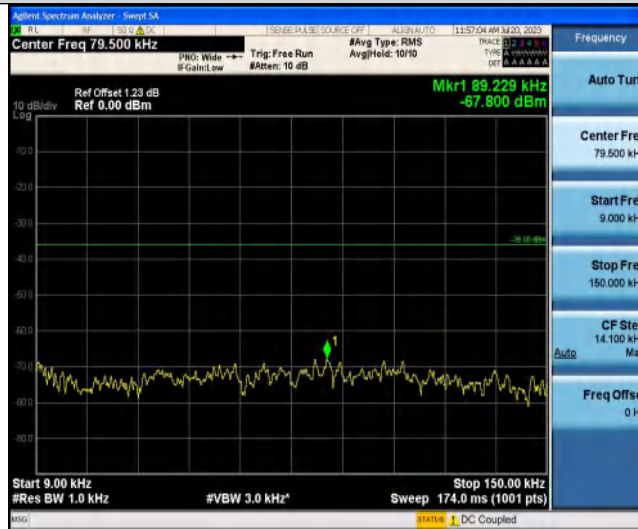
NTNV-Band3-1.4MHz-QPSK-19943-1RB#5-0.15~30-10-30
