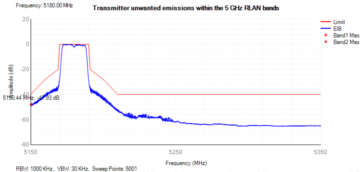
Tx. Emissions EIB NVNT 802.11a 5180MHz Sub Band1
