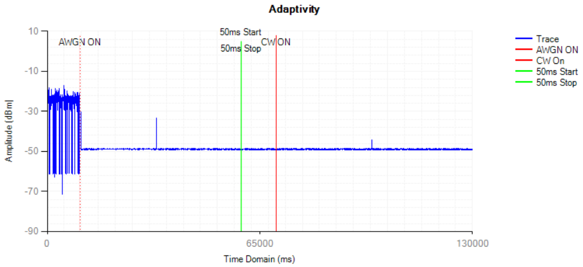
Control Signal NVNT 802.11g 2412MHz
