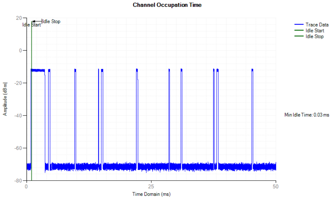
COT NVNT 802.11n(HT20) 2472MHz
