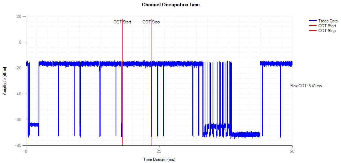
Idle NVNT 802.11n(HT40) 2462MHz
