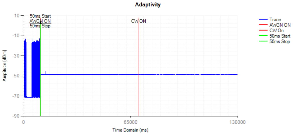
Control Signal NVNT 802.11n(HT20) 2472MHz
