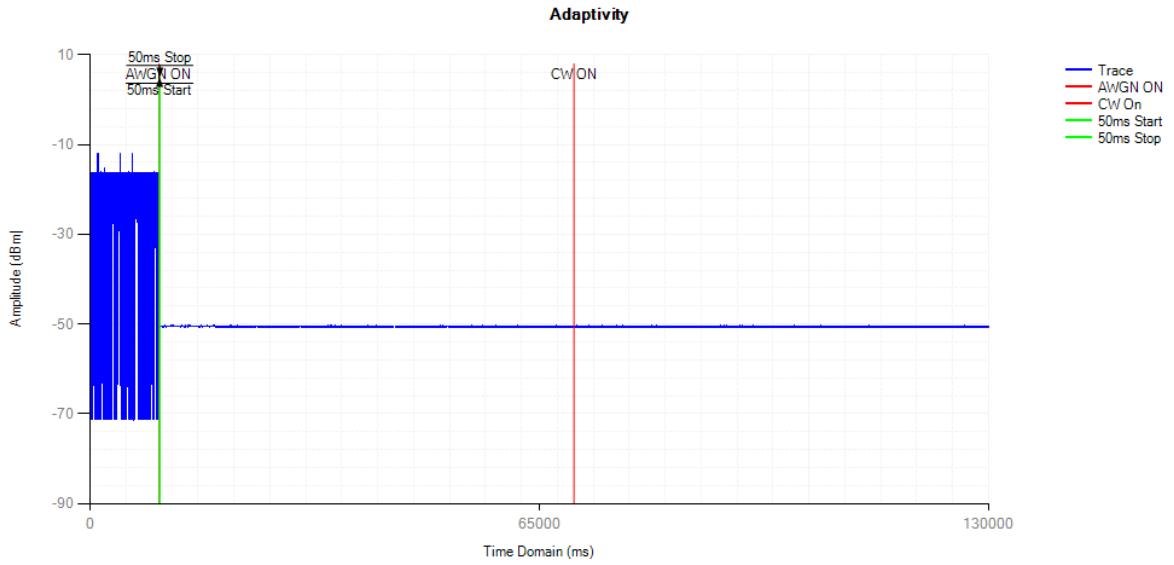
Control Signal NVNT 802.11n(HT40) 2462MHz
