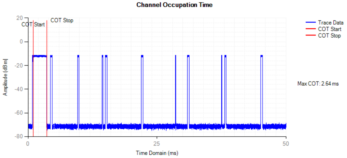
Idle NVNT 802.11n(HT20) 2412MHz
