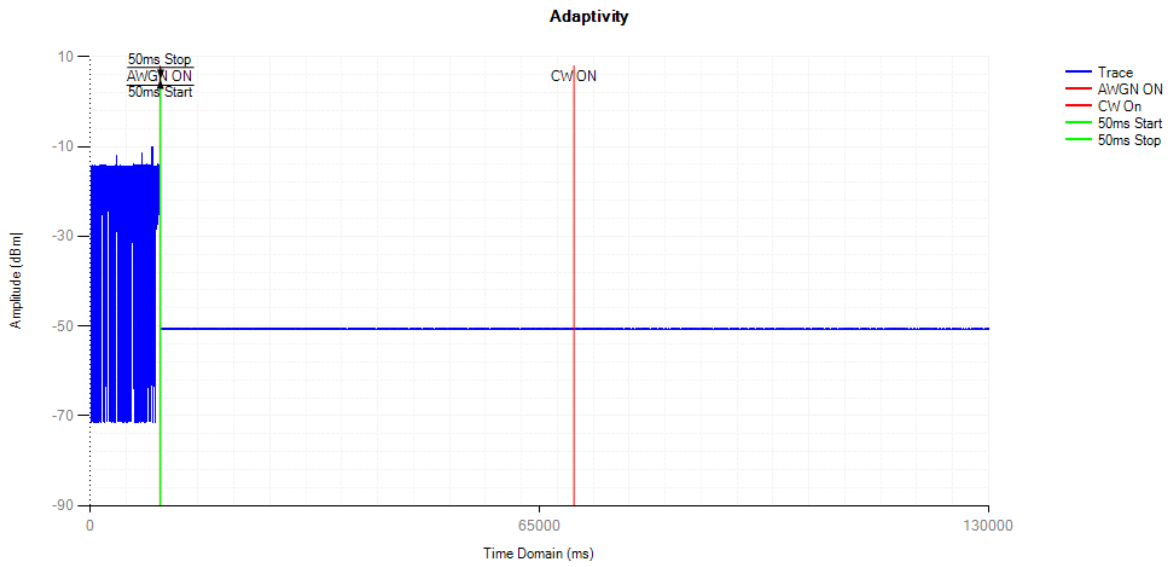
Control Signal NVNT 802.11n(HT40) 2422MHz
