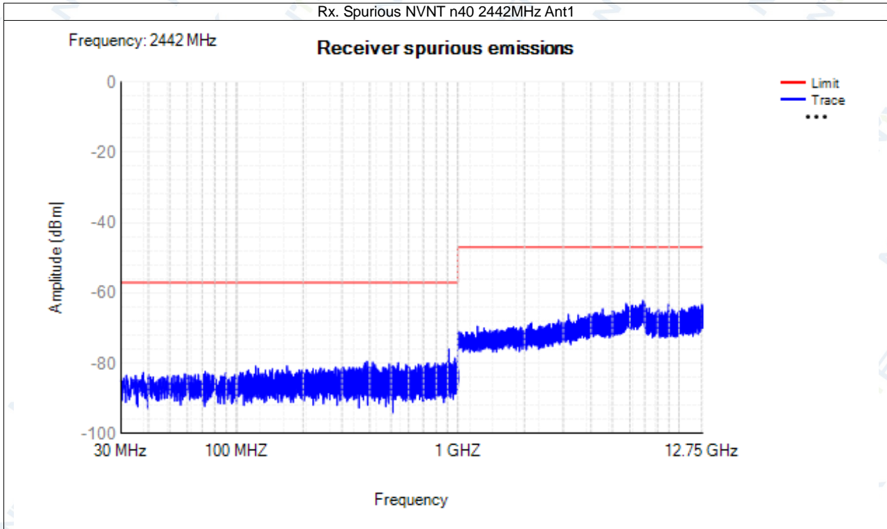
Rx. Spurious NVNT n40 2462MHz Ant1
