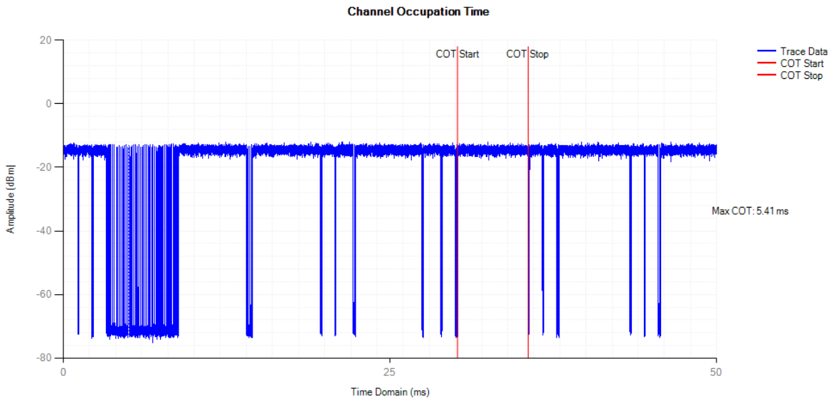
Idle NVNT 802.11n(HT40) 2422MHz
