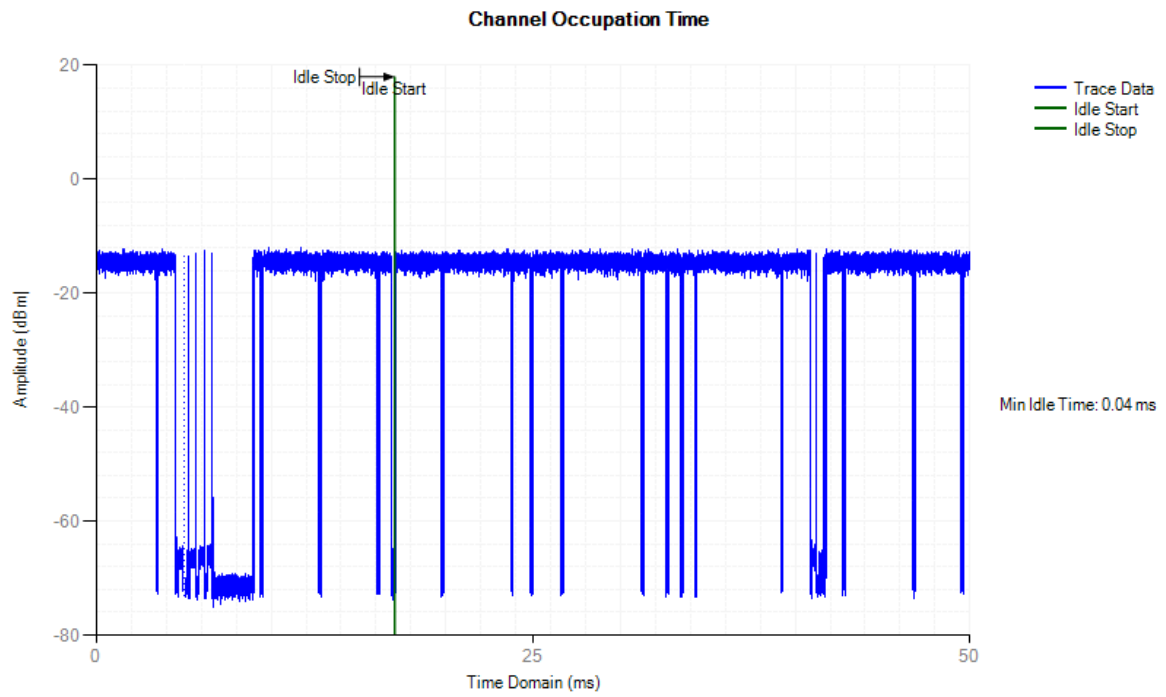
COT NVNT 802.11n(HT40) 2462MHz
