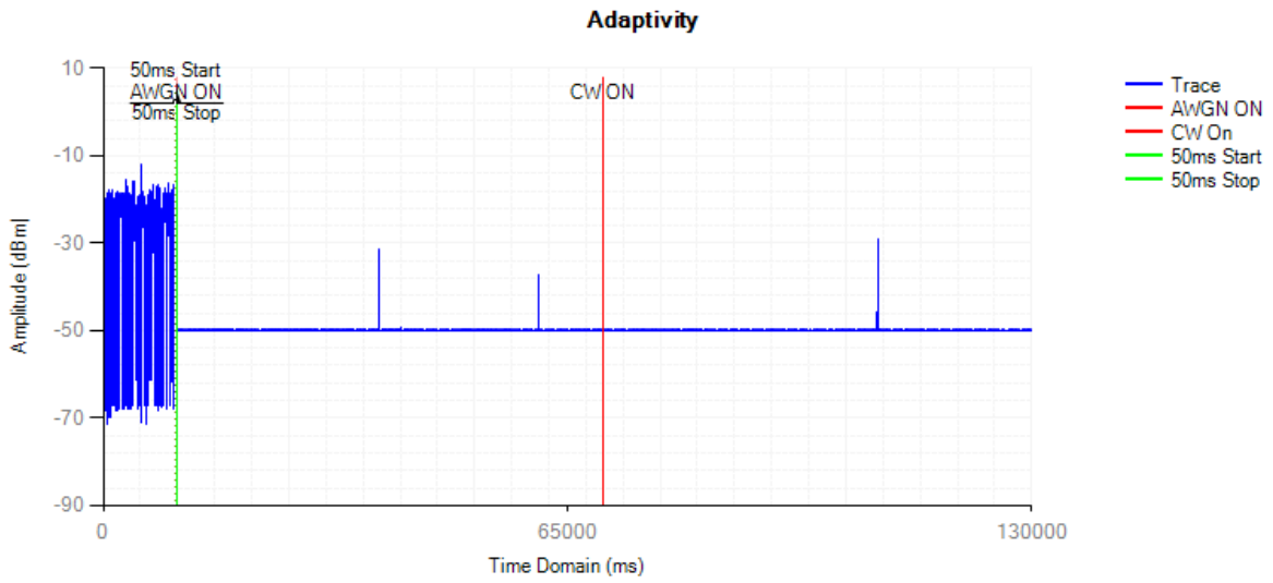
Control Signal NVNT 802.11g 2472MHz
