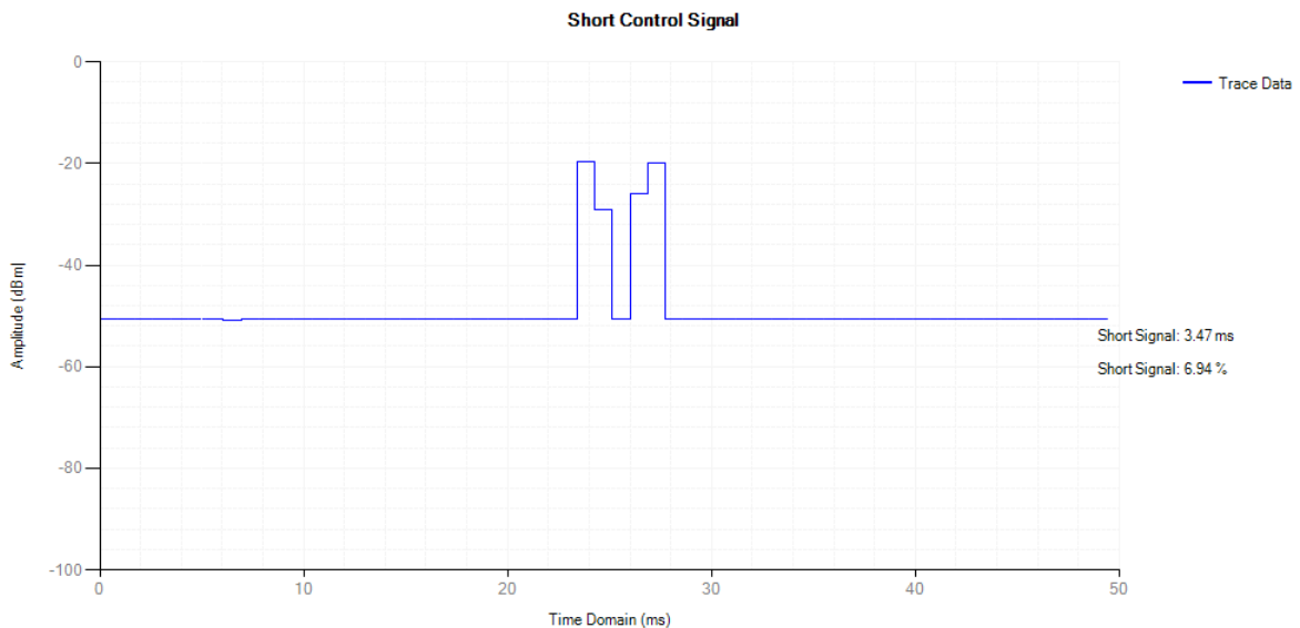
Adaptivity NVNT 802.11b 2472MHz
