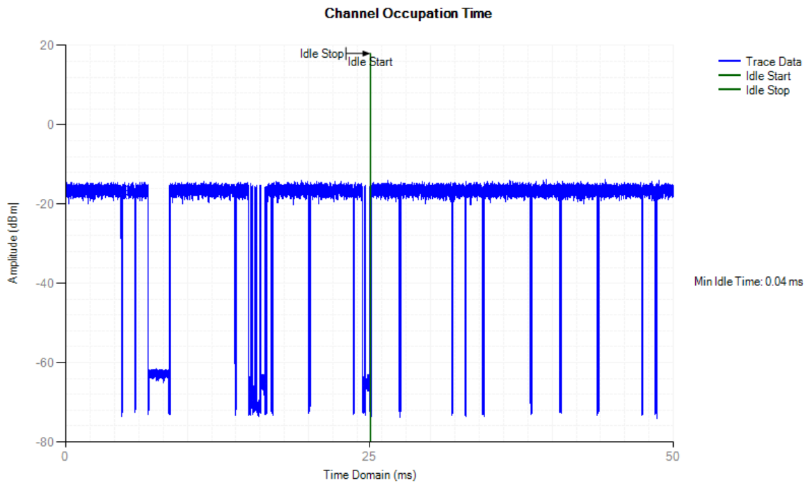
Idle NVNT 802.11n(HT40) 2462MHz
