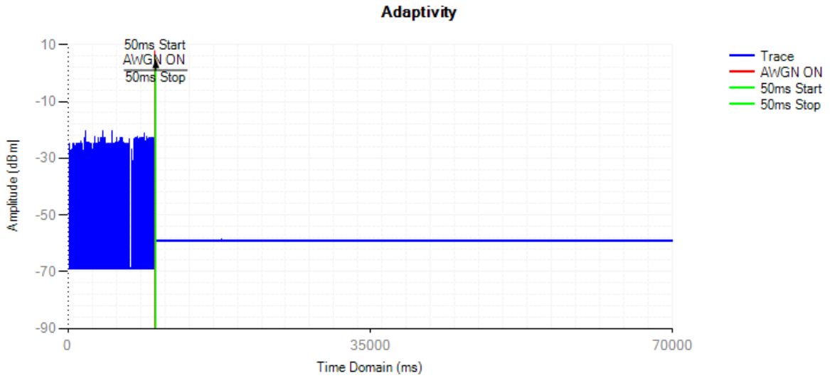
Control Signal NVNT 802.11n(HT40) 5190MHz AWGN
