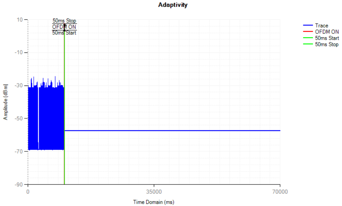
Control Signal NVNT 802.11ac80 5210MHz OFDM
