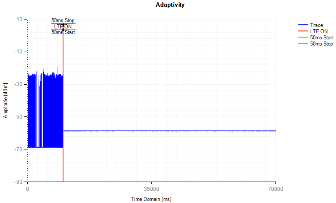
Control Signal NVNT 802.11n(HT40) 5190MHz LTE
