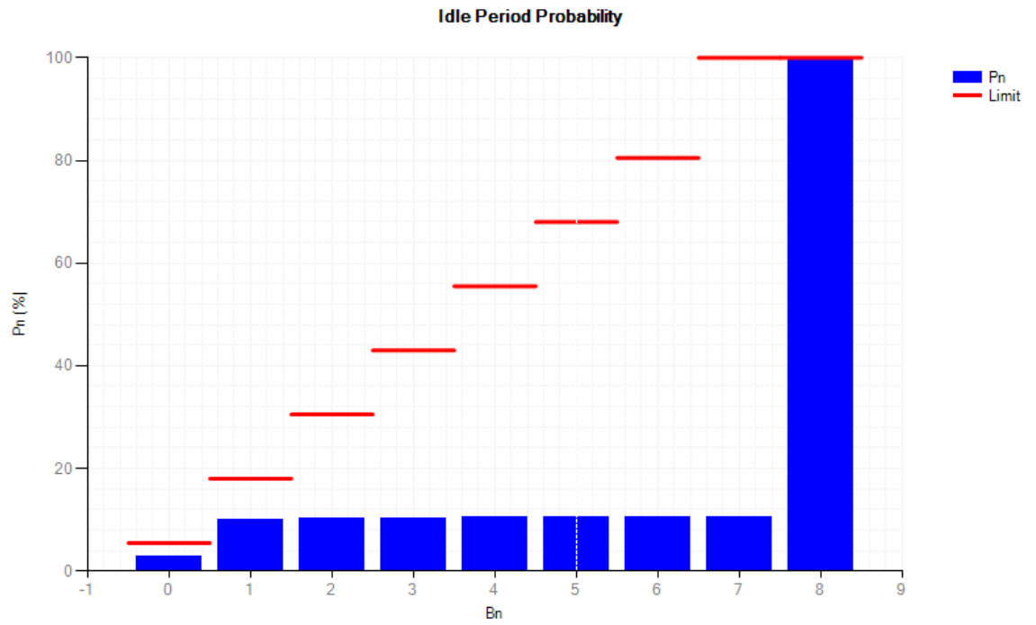
Idle Period Probability NVNT 802.11n(HT40) 5190MHz
