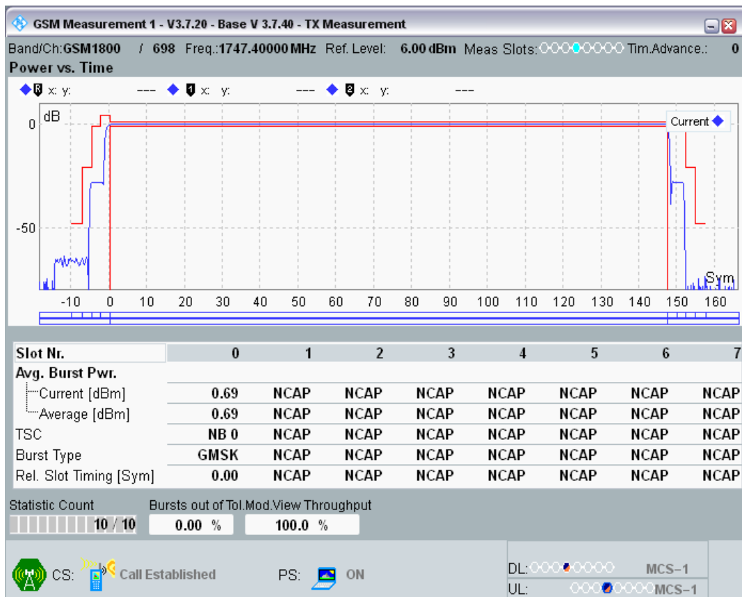
GSM1800 Channel=698 PCL=14
