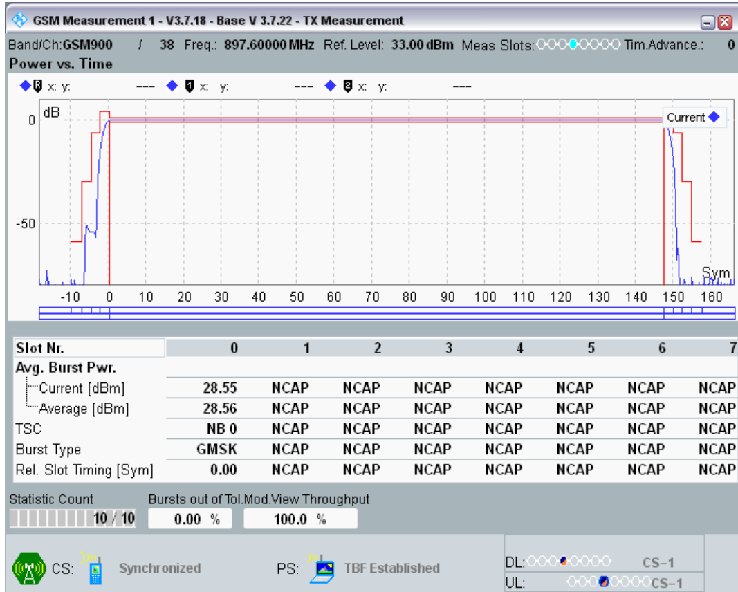
GPRS900 Channel=38 Gamma=7;7;7
