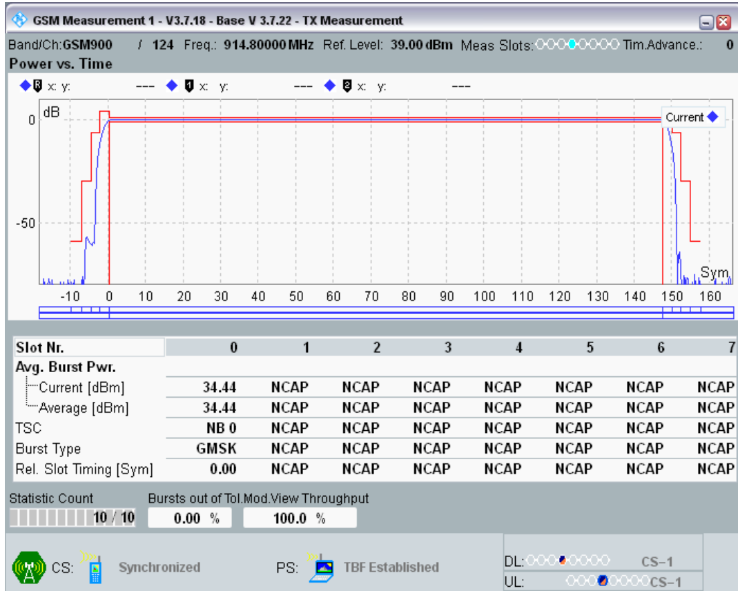
GPRS900 Channel=124 Gamma=4;4;4;4
