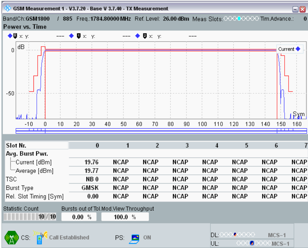
GSM1800 Channel=885 PCL=4
