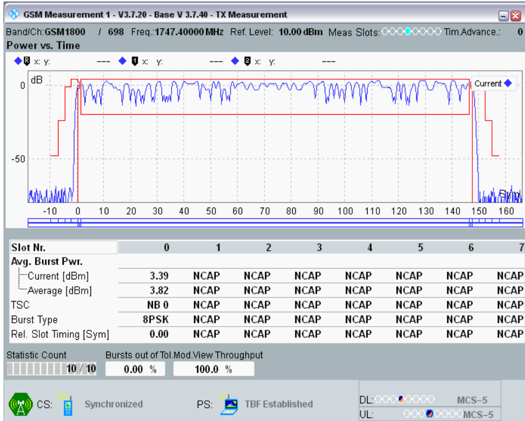
EGPRS1800 Channel=698 Gamma=7;7;7;7
