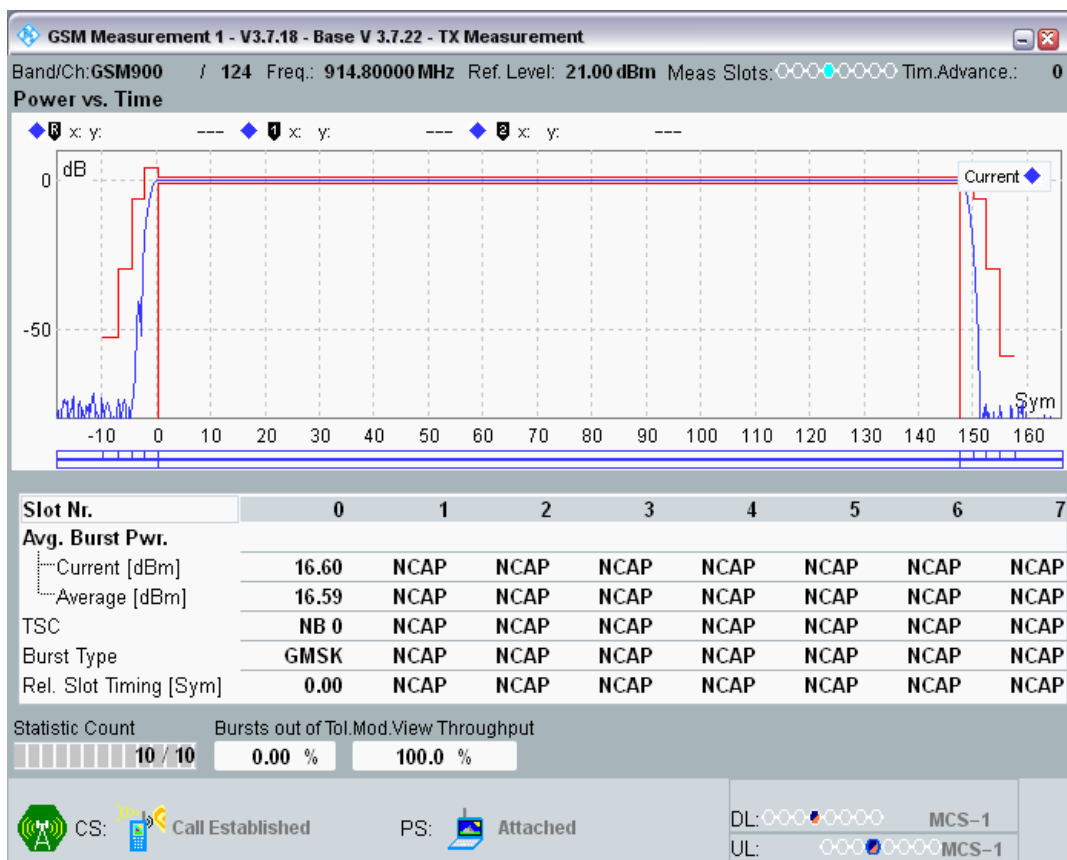
GSM900 Channel=124 PCL=15
