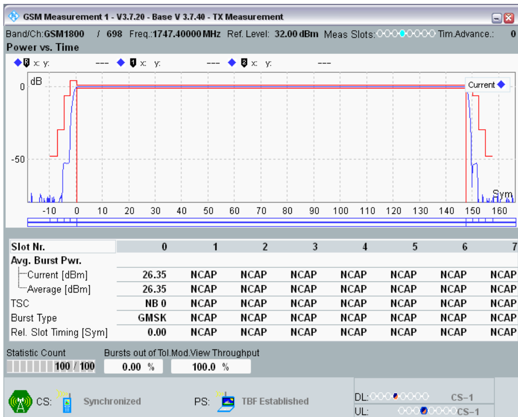
GPRS1800 Channel=698 Gamma=4;4;4;4
