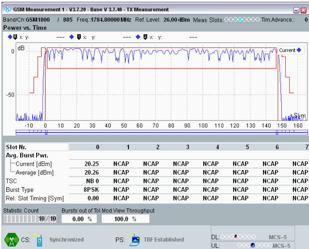
EGPRS1800 Channel=885 Gamma=7;7;7;7
