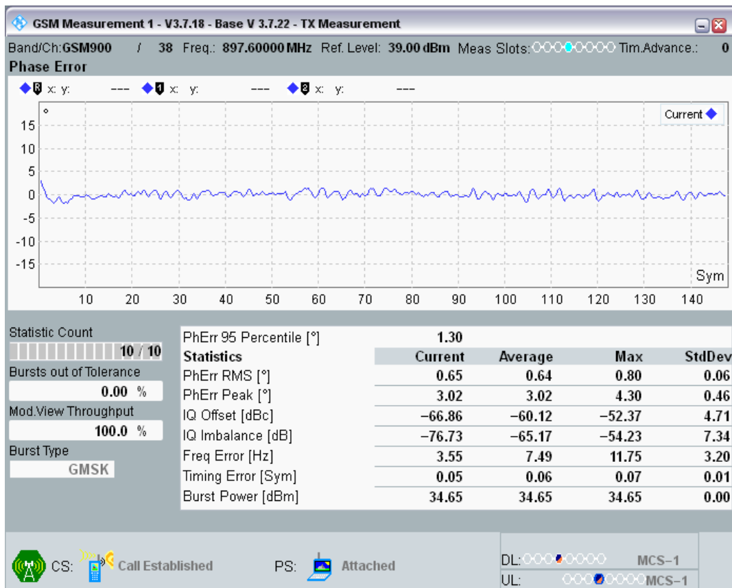
GSM900 Channel=38 PCL=5 TU3 @1
