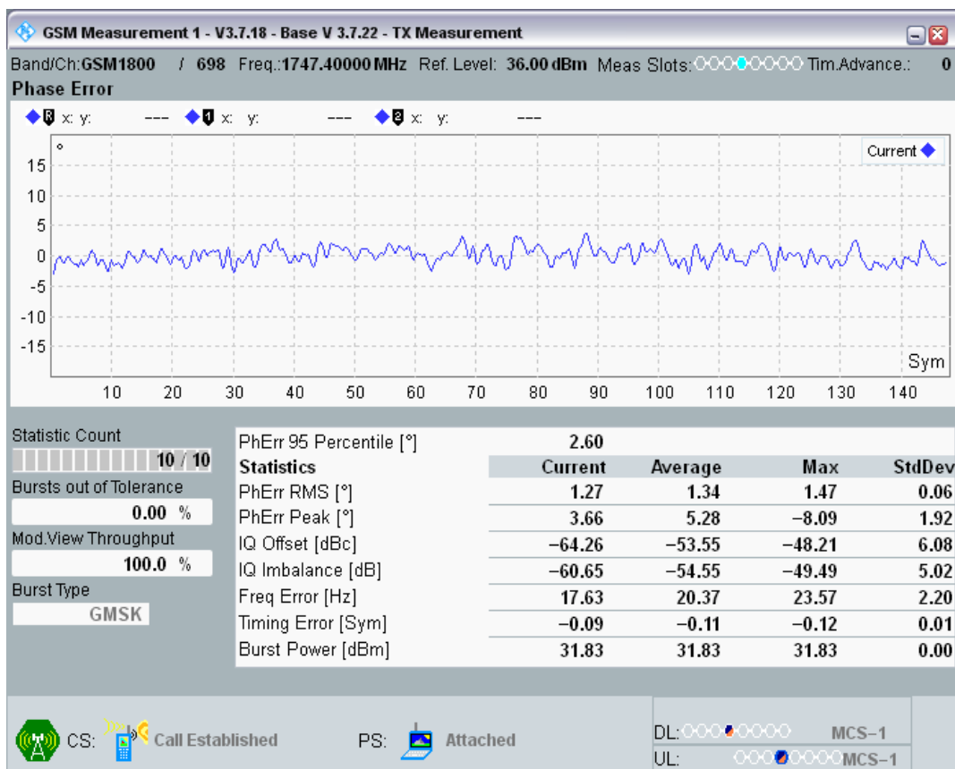
GSM1800 Channel=698 PCL=0 TU1_5 @11
