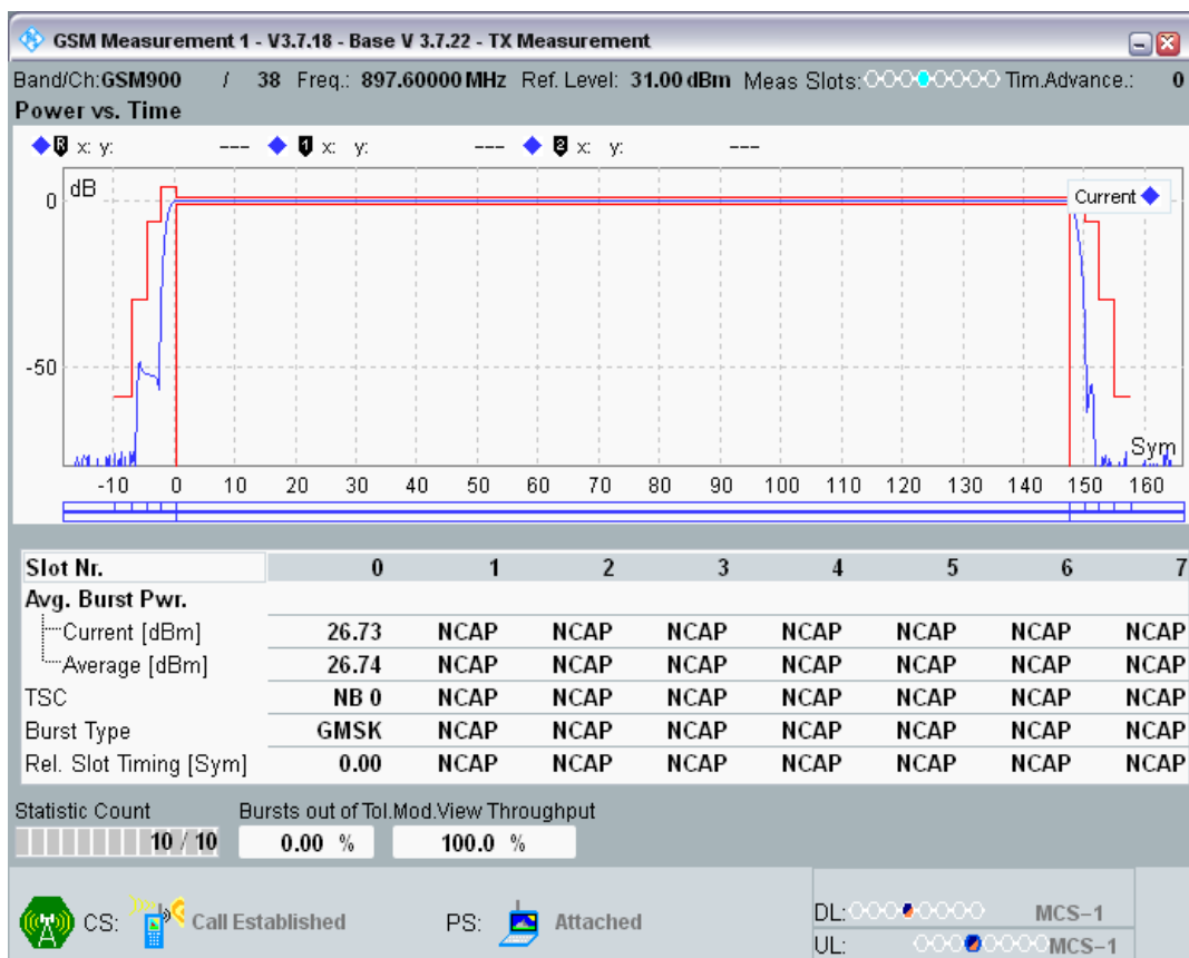
GSM900 Channel=38 PCL=10
