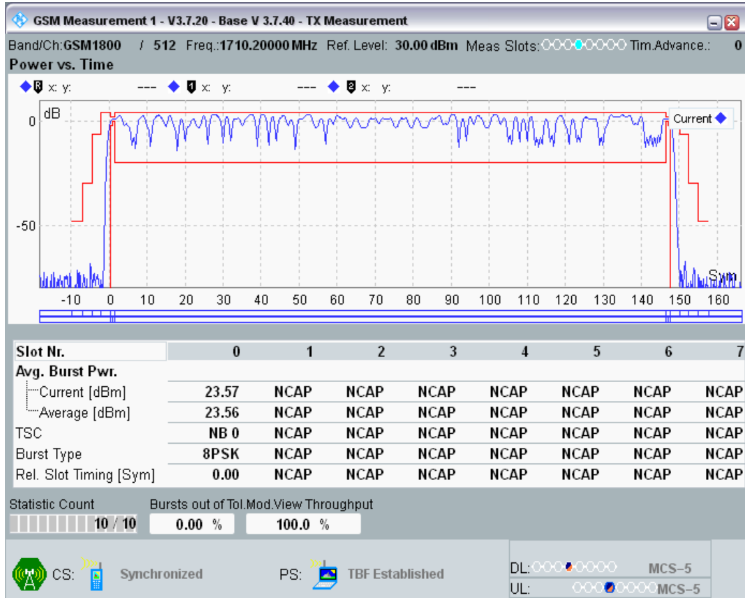
EGPRS1800 Channel=512 Gamma=7;7;7;7
