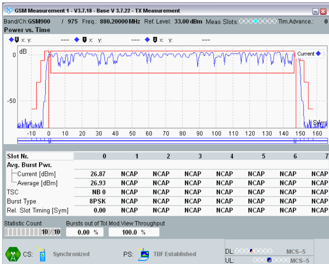
EGPRS900 Channel=975 Gamma=7;7;7;7
