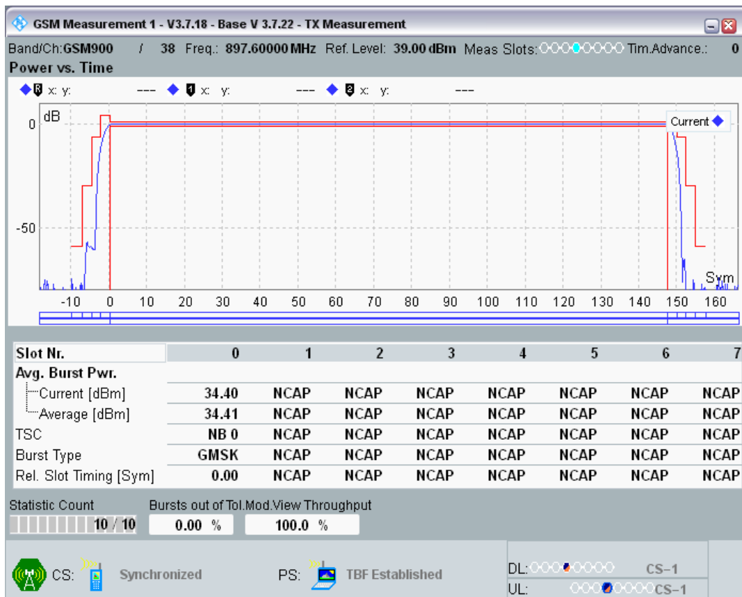
GPRS900 Channel=38 Gamma=4;4;4;4
