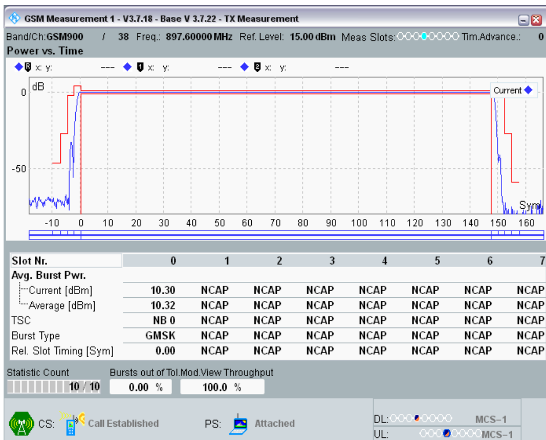
GSM900 Channel=38 PCL=18
