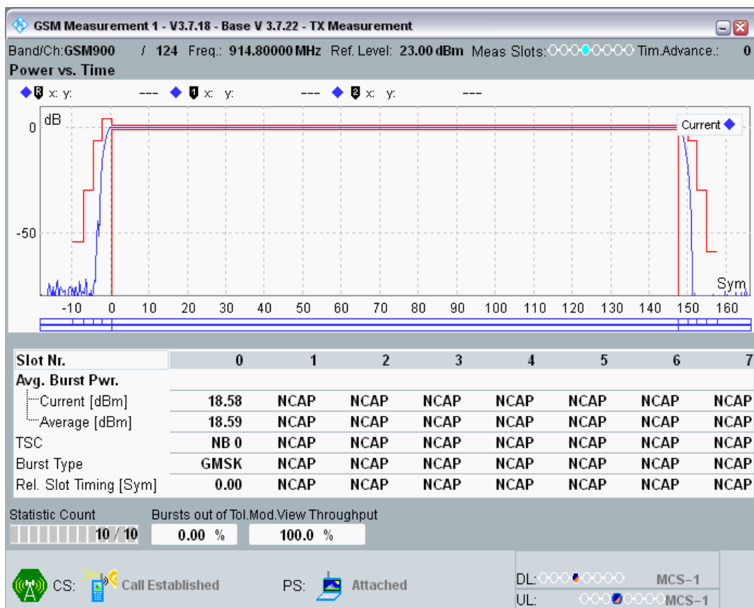
GSM900 Channel=124 PCL=14
