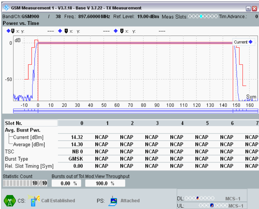
GSM900 Channel=38 PCL=16
