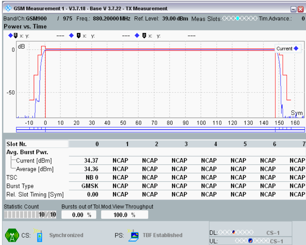
GPRS900 Channel=975 Gamma=4;4;4;4
