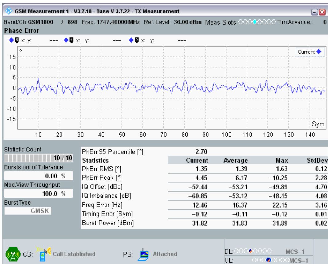
GSM1800 Channel=698 PCL=0 TU1_5 @17
