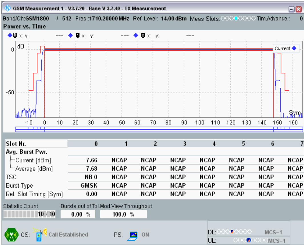
GSM1800 Channel=512 PCL=8
