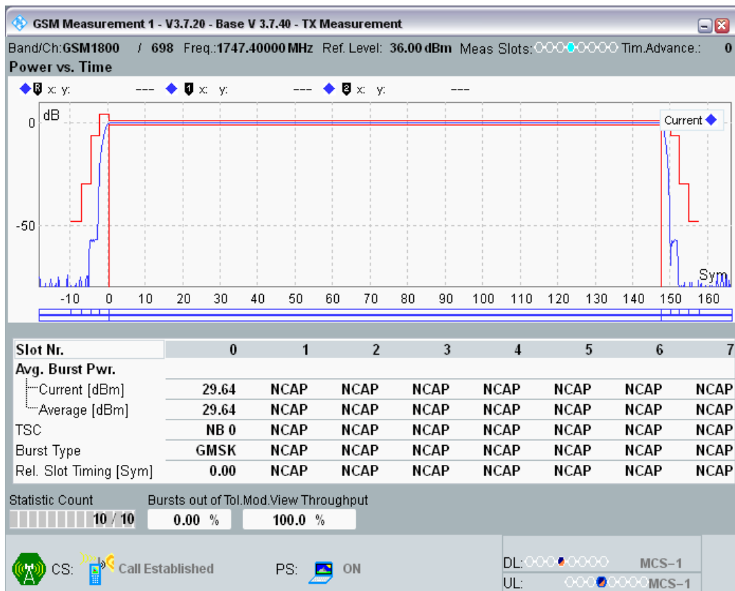
GSM1800 Channel=512 PCL=6
