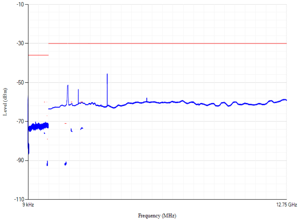
WCDMA Band1 Channel=9612 MBW 0kHz
